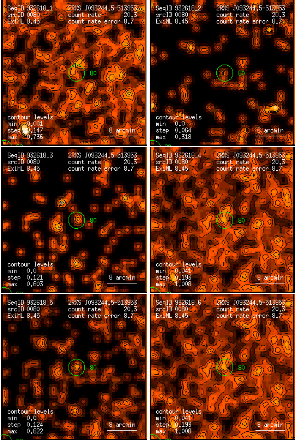
Figure 80: RASS 932618: detection 0080: band rate images, Gaussian filter: (1) PSPC channels 11 – 41, (2) 52 – 90, (3) 91 – 201, (4) 11 – 235, (5) 52 – 201, (6) 11 – 201. Broad band rates in counts/ks. Band rate contour levels in counts/ks/arcmin 2 .
