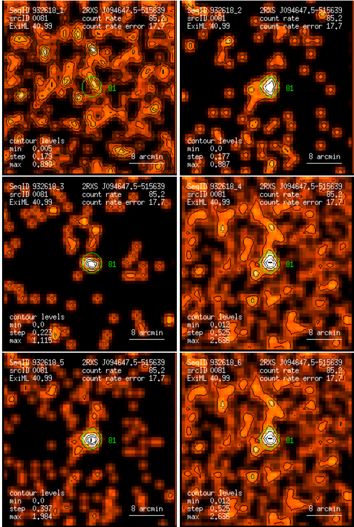
Figure 81: RASS 932618: detection 0081: band rate images, Gaussian filter: (1) PSPC channels 11 – 41, (2) 52 – 90, (3) 91 – 201, (4) 11 – 235, (5) 52 – 201, (6) 11 – 201. Broad band rates in counts/ks. Band rate contour levels in counts/ks/arcmin 2 .
