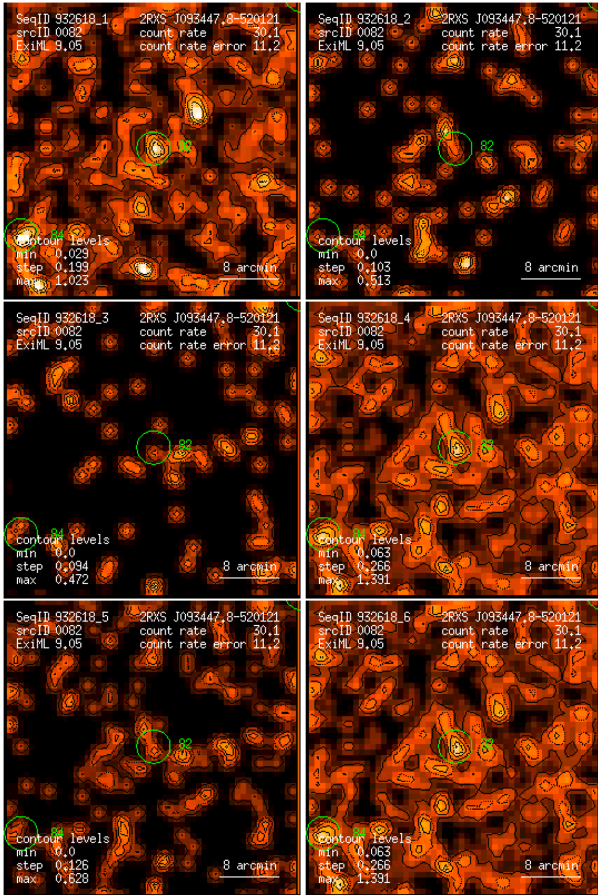
Figure 82: RASS 932618: detection 0082: band rate images, Gaussian filter: (1) PSPC channels 11 – 41, (2) 52 – 90, (3) 91 – 201, (4) 11 – 235, (5) 52 – 201, (6) 11 – 201. Broad band rates in counts/ks. Band rate contour levels in counts/ks/arcmin 2 .
