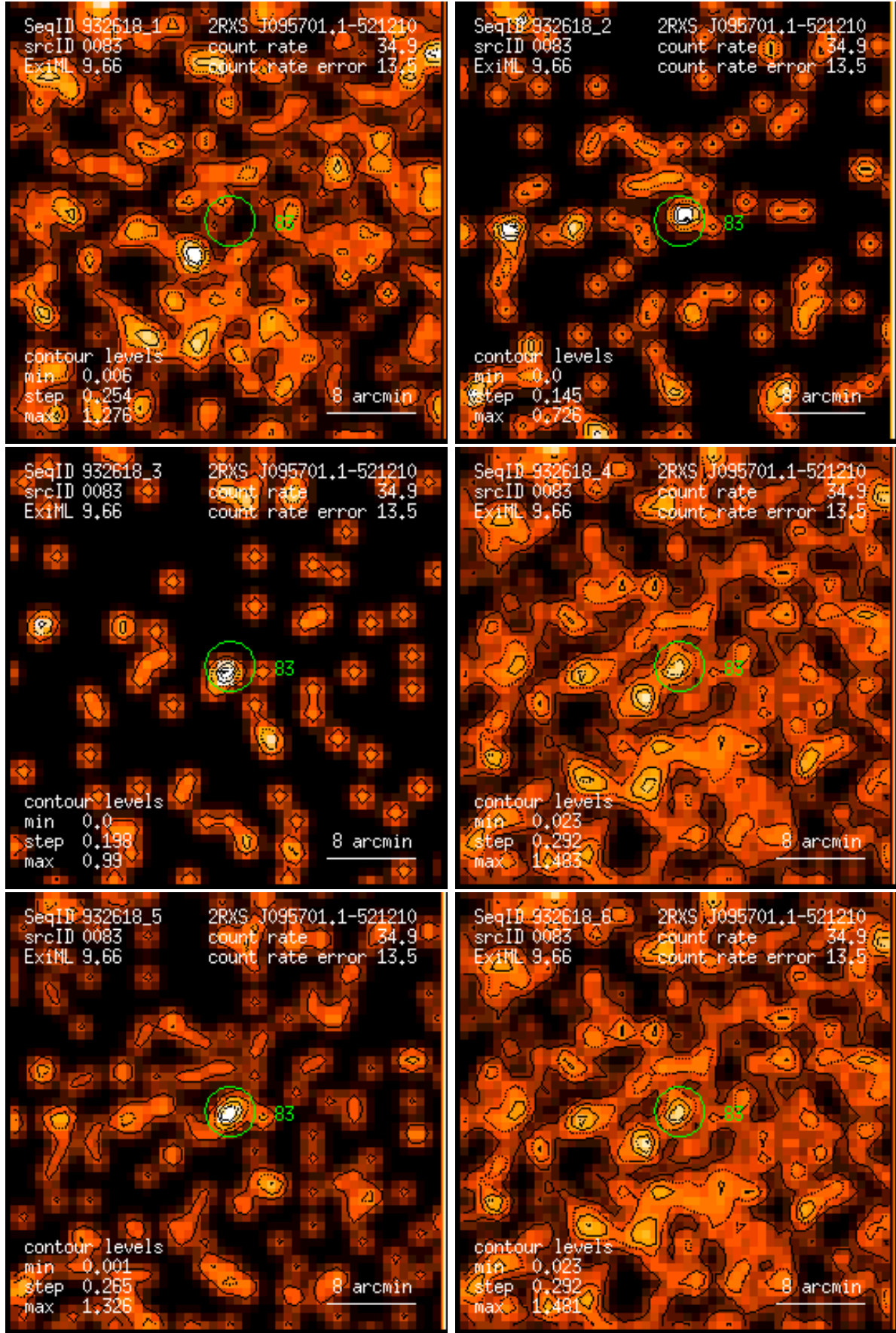
Figure 83: RASS 932618: detection 0083: band rate images, Gaussian filter: (1) PSPC channels 11 – 41, (2) 52 – 90, (3) 91 – 201, (4) 11 – 235, (5) 52 – 201, (6) 11 – 201. Broad band rates in counts/ks. Band rate contour levels in counts/ks/arcmin 2 .
