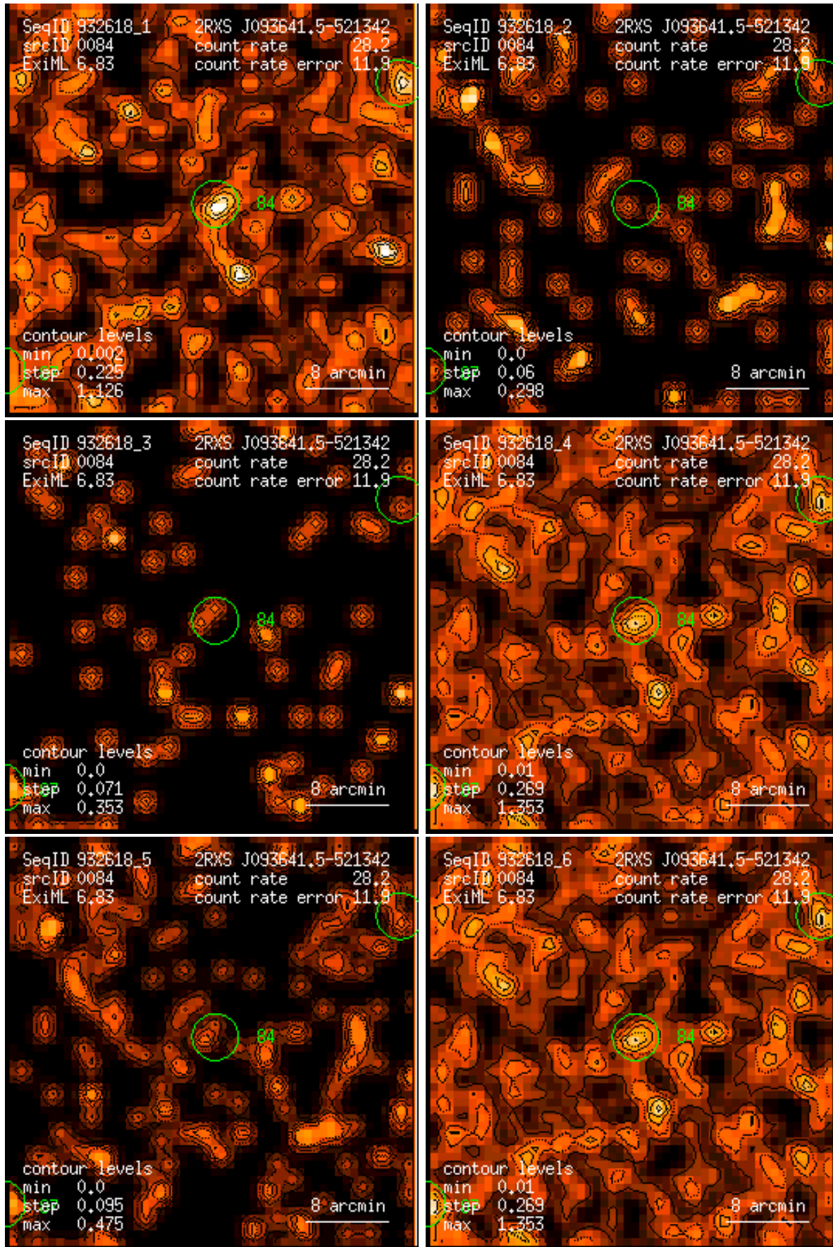
Figure 84: RASS 932618: detection 0084: band rate images, Gaussian filter: (1) PSPC channels 11 – 41, (2) 52 – 90, (3) 91 – 201, (4) 11 – 235, (5) 52 – 201, (6) 11 – 201. Broad band rates in counts/ks. Band rate contour levels in counts/ks/arcmin 2 .
