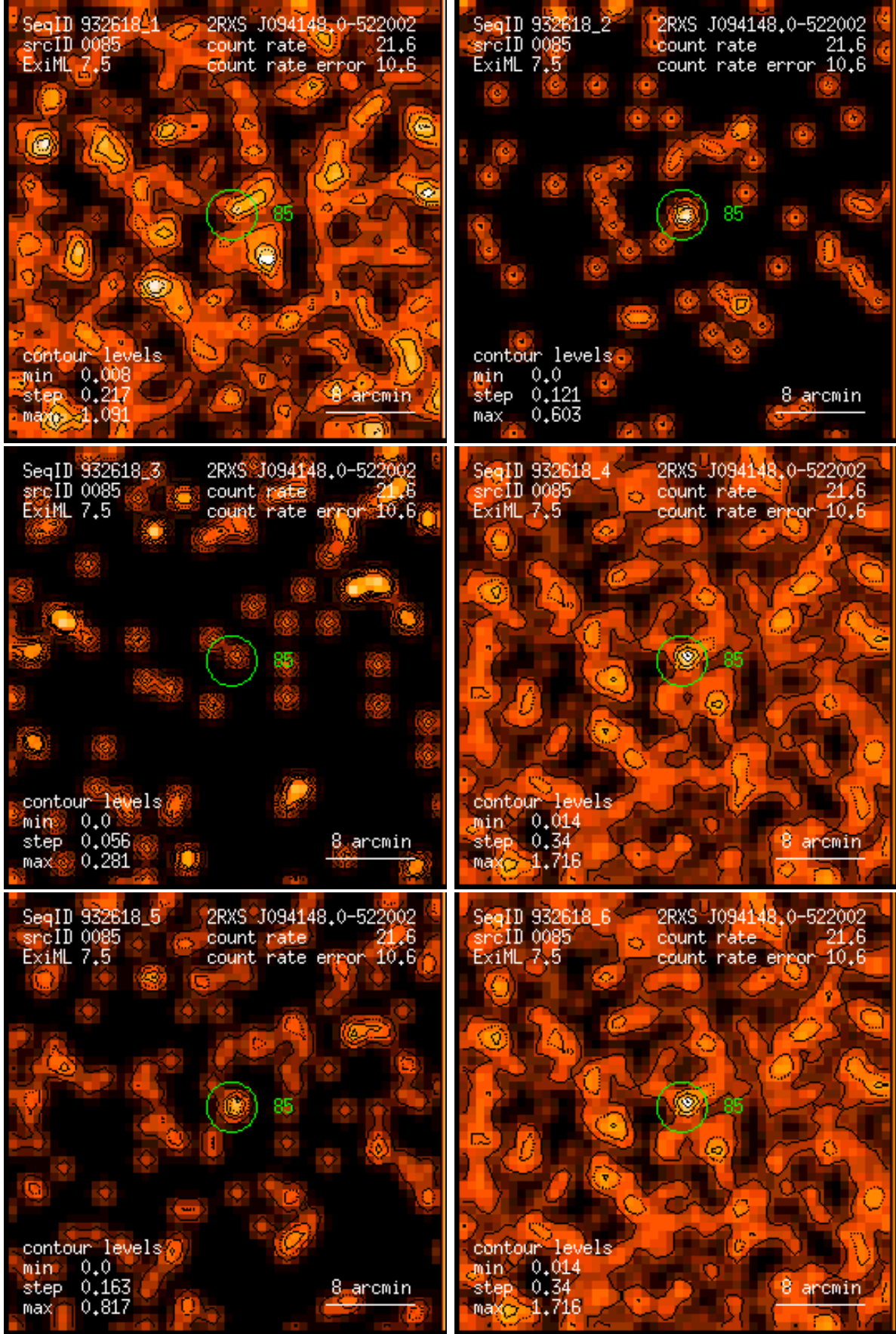
Figure 85: RASS 932618: detection 0085: band rate images, Gaussian filter: (1) PSPC channels 11 – 41, (2) 52 – 90, (3) 91 – 201, (4) 11 – 235, (5) 52 – 201, (6) 11 – 201. Broad band rates in counts/ks. Band rate contour levels in counts/ks/arcmin 2 .
