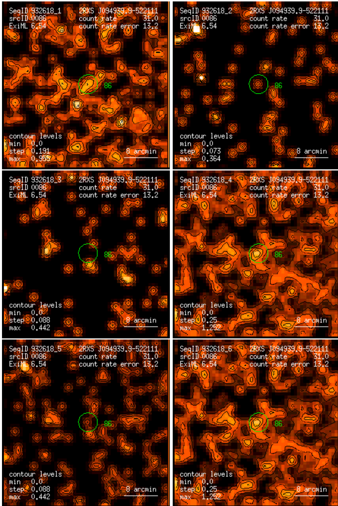
Figure 86: RASS 932618: detection 0086: band rate images, Gaussian filter: (1) PSPC channels 11 – 41, (2) 52 – 90, (3) 91 – 201, (4) 11 – 235, (5) 52 – 201, (6) 11 – 201. Broad band rates in counts/ks. Band rate contour levels in counts/ks/arcmin 2 .
