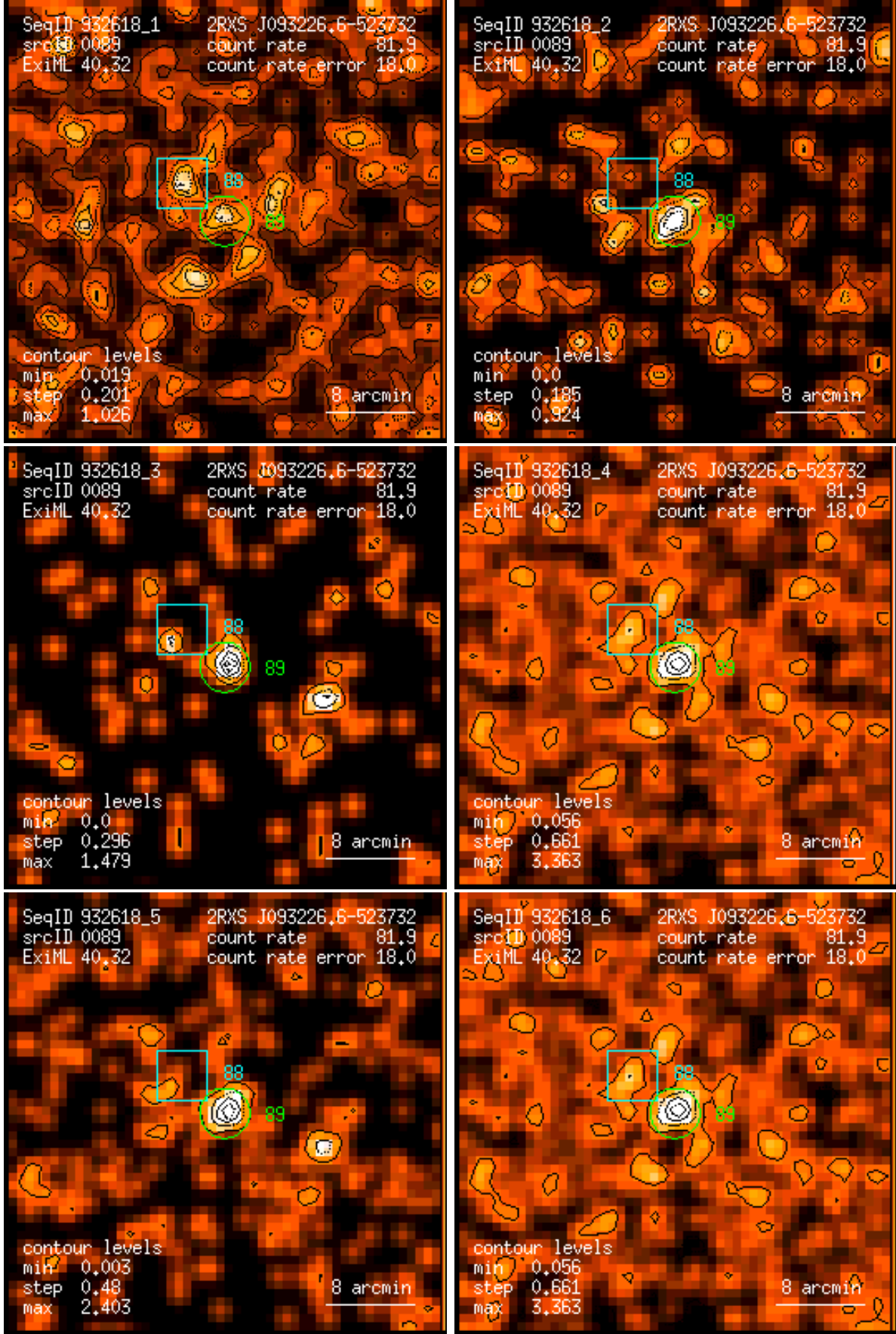
Figure 89: RASS 932618: detection 0089: band rate images, Gaussian filter: (1) PSPC channels 11 – 41, (2) 52 – 90, (3) 91 – 201, (4) 11 – 235, (5) 52 – 201, (6) 11 – 201. Broad band rates in counts/ks. Band rate contour levels in counts/ks/arcmin 2 .
