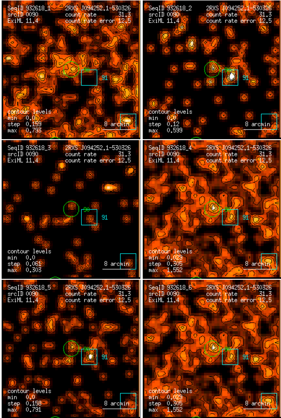
Figure 90: RASS 932618: detection 0090: band rate images, Gaussian filter: (1) PSPC channels 11 – 41, (2) 52 – 90, (3) 91 – 201, (4) 11 – 235, (5) 52 – 201, (6) 11 – 201. Broad band rates in counts/ks. Band rate contour levels in counts/ks/arcmin 2 .
