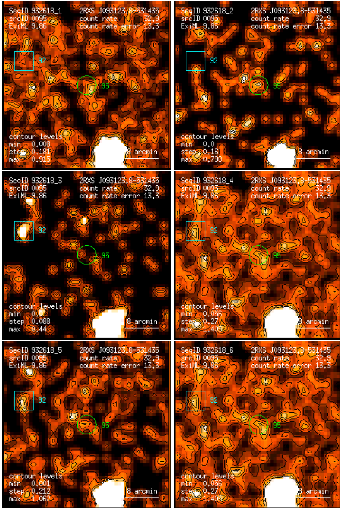
Figure 95: RASS 932618: detection 0095: band rate images, Gaussian filter: (1) PSPC channels 11 – 41, (2) 52 – 90, (3) 91 – 201, (4) 11 – 235, (5) 52 – 201, (6) 11 – 201. Broad band rates in counts/ks. Band rate contour levels in counts/ks/arcmin 2 .
