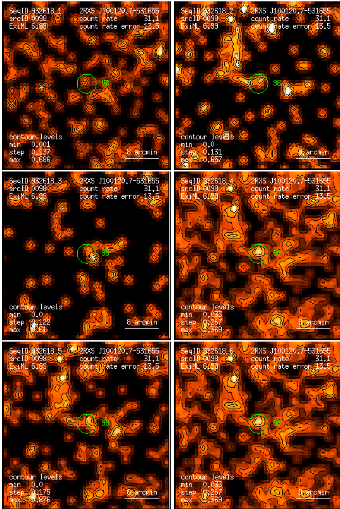
Figure 98: RASS 932618: detection 0098: band rate images, Gaussian filter: (1) PSPC channels 11 – 41, (2) 52 – 90, (3) 91 – 201, (4) 11 – 235, (5) 52 – 201, (6) 11 – 201. Broad band rates in counts/ks. Band rate contour levels in counts/ks/arcmin 2 .
