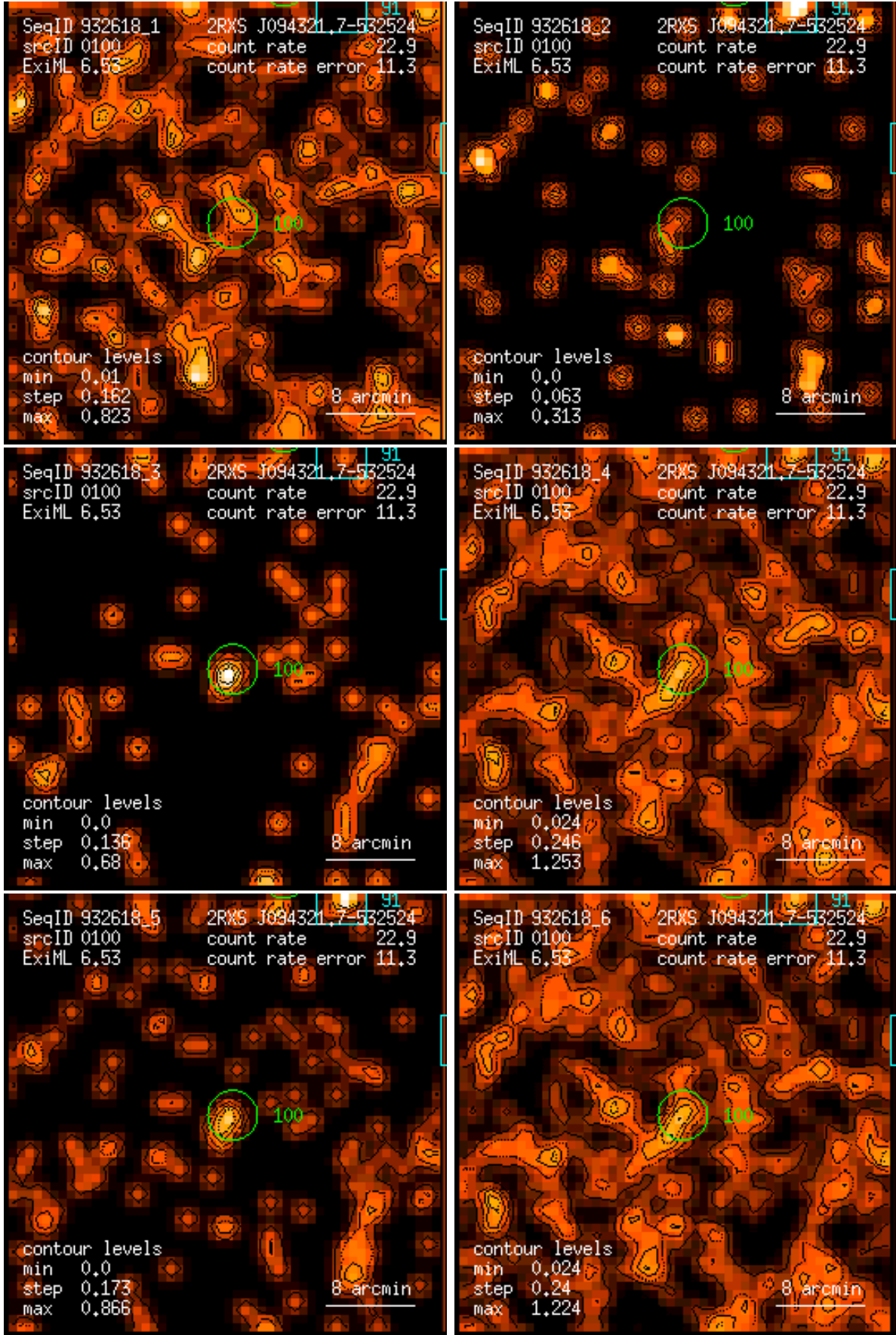
Figure 100: RASS 932618: detection 0100: band rate images, Gaussian filter: (1) PSPC channels 11 – 41, (2) 52 – 90, (3) 91 – 201, (4) 11 – 235, (5) 52 – 201, (6) 11 – 201. Broad band rates in counts/ks. Band rate contour levels in counts/ks/arcmin 2 .
