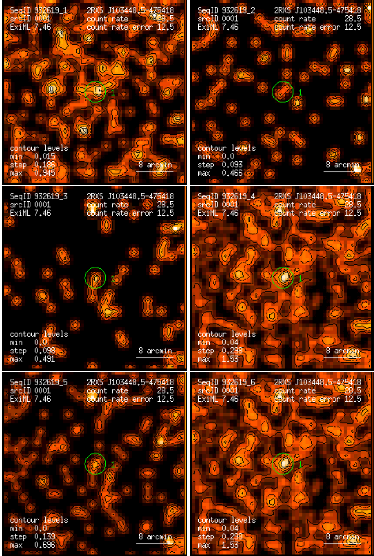
Figure 1: RASS 932619: detection 0001: band rate images, Gaussian filter: (1) PSPC channels 11 – 41, (2) 52 – 90, (3) 91 – 201, (4) 11 – 235, (5) 52 – 201, (6) 11 – 201. Broad band rates in counts/ks. Band rate contour levels in counts/ks/arcmin 2 .
