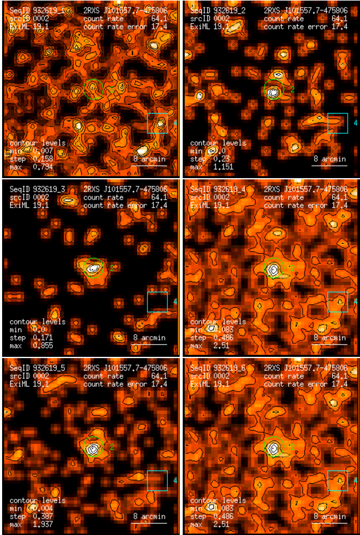
Figure 2: RASS 932619: detection 0002: band rate images, Gaussian filter: (1) PSPC channels 11 – 41, (2) 52 – 90, (3) 91 – 201, (4) 11 – 235, (5) 52 – 201, (6) 11 – 201. Broad band rates in counts/ks. Band rate contour levels in counts/ks/arcmin 2 .
