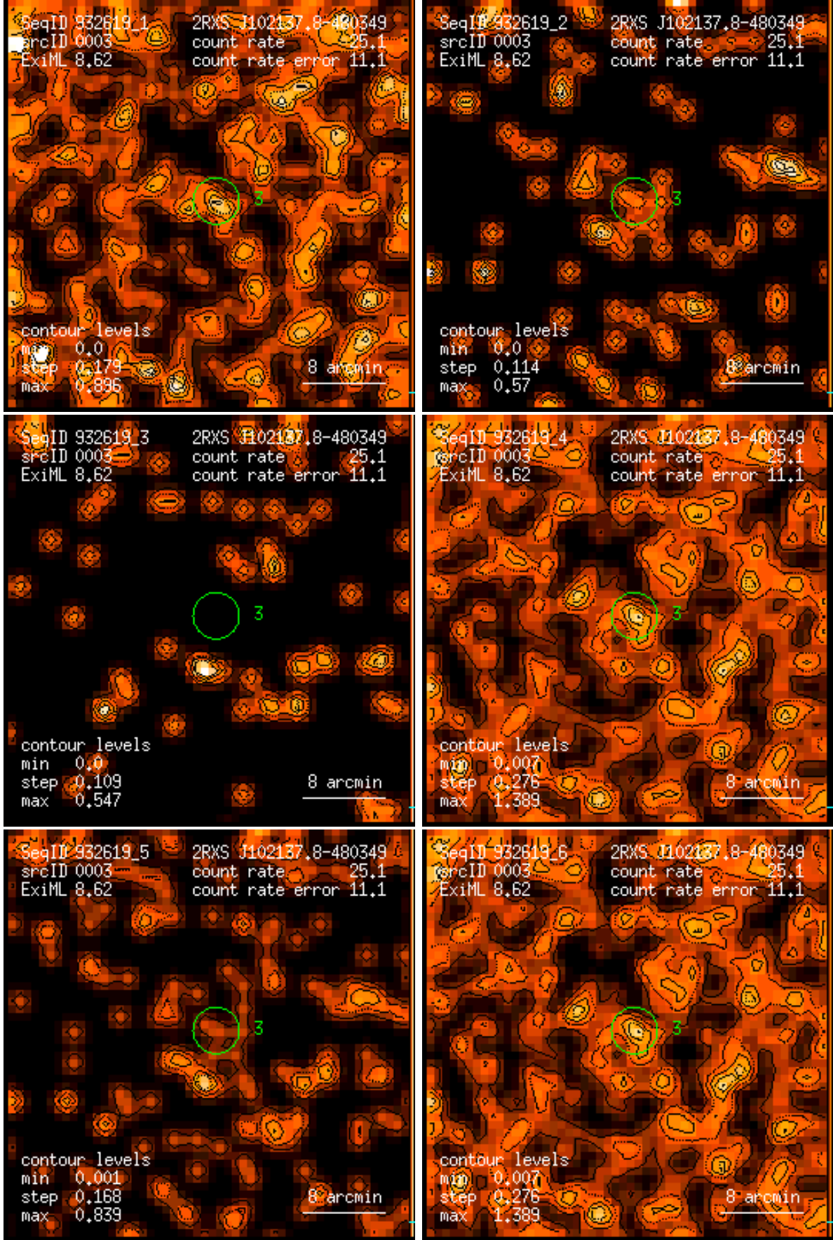
Figure 3: RASS 932619: detection 0003: band rate images, Gaussian filter: (1) PSPC channels 11 – 41, (2) 52 – 90, (3) 91 – 201, (4) 11 – 235, (5) 52 – 201, (6) 11 – 201. Broad band rates in counts/ks. Band rate contour levels in counts/ks/arcmin 2 .
