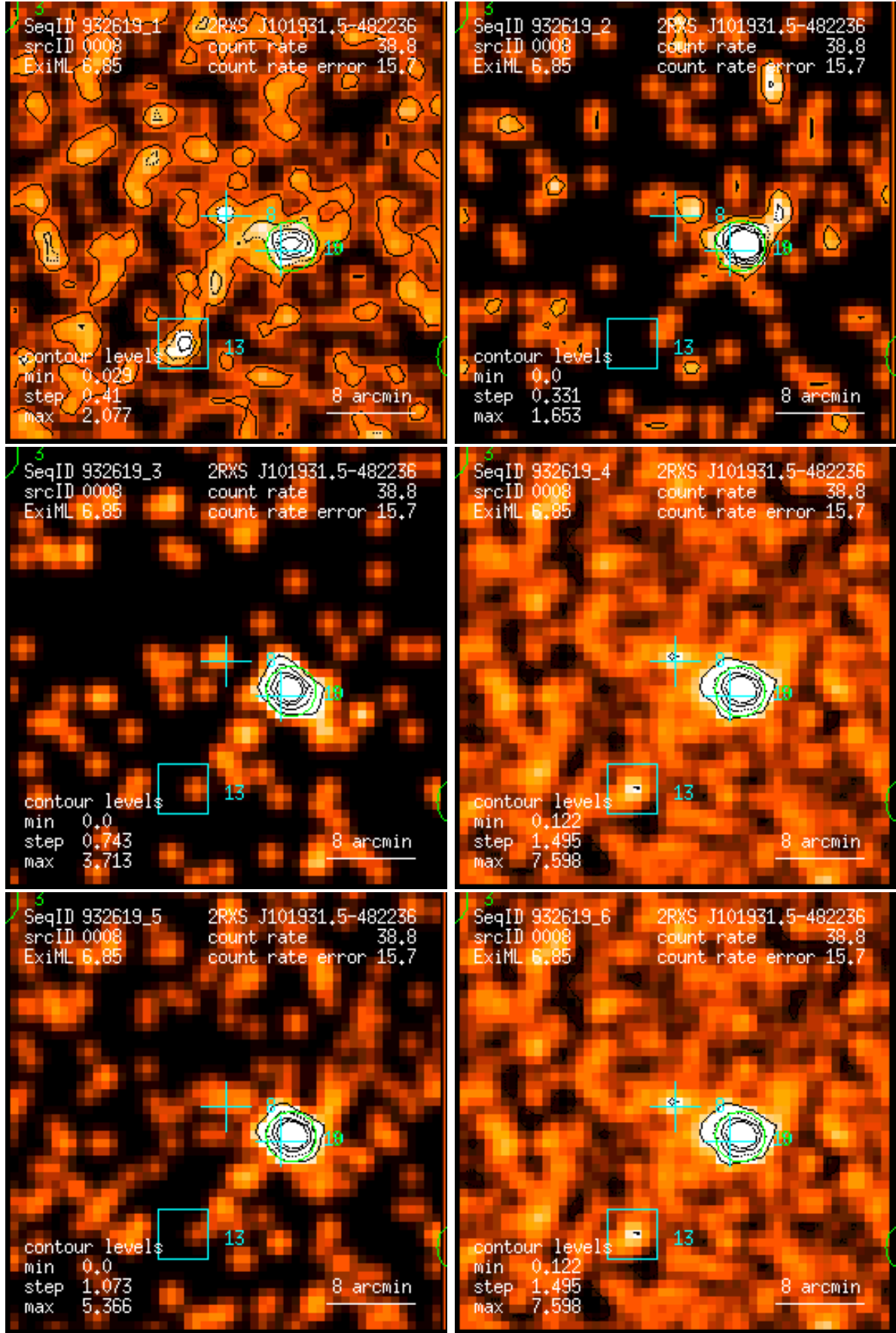
Figure 8: RASS 932619: detection 0008: band rate images, Gaussian filter: (1) PSPC channels 11 – 41, (2) 52 – 90, (3) 91 – 201, (4) 11 – 235, (5) 52 – 201, (6) 11 – 201. Broad band rates in counts/ks. Band rate contour levels in counts/ks/arcmin 2 .
