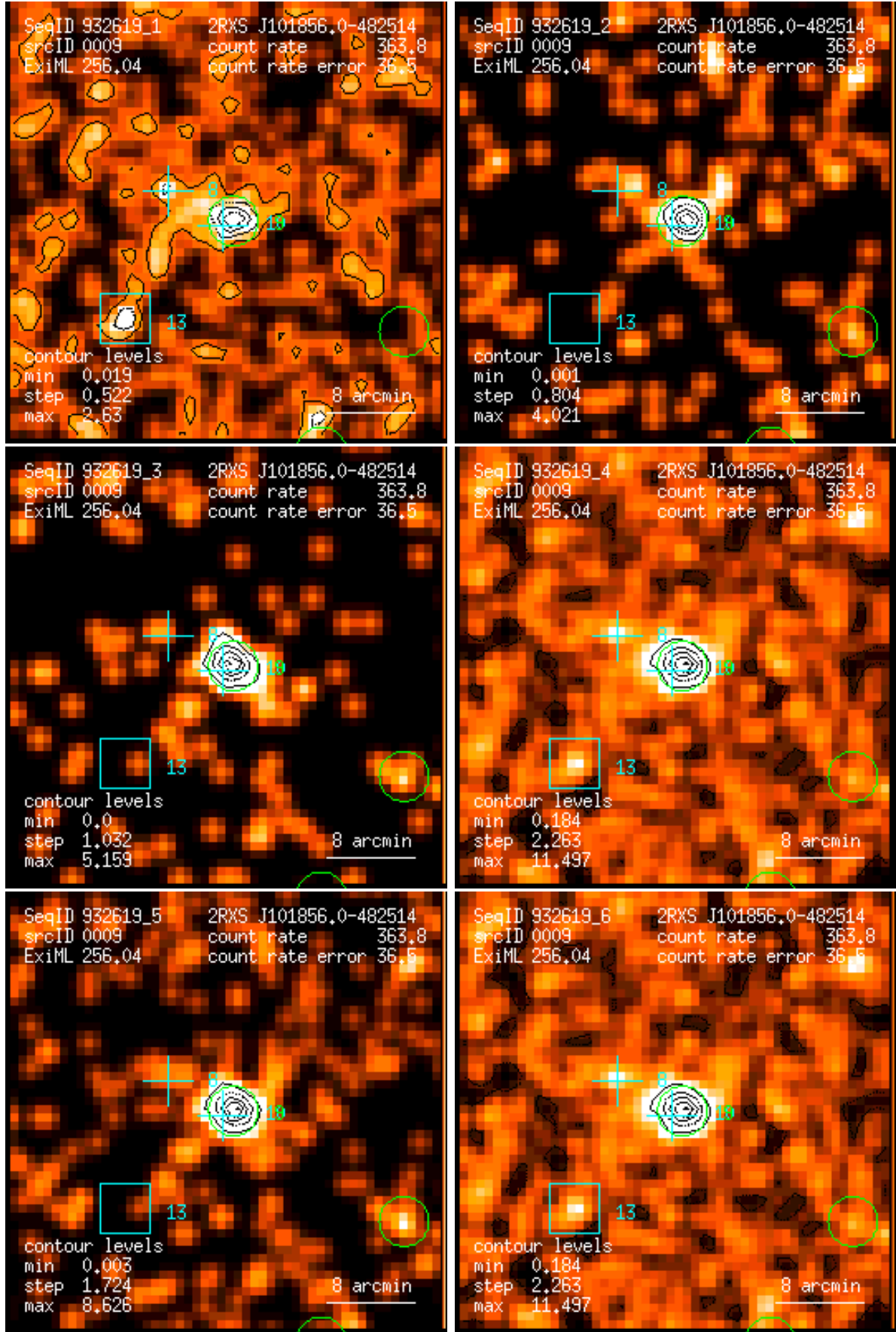
Figure 9: RASS 932619: detection 0009: band rate images, Gaussian filter: (1) PSPC channels 11 – 41, (2) 52 – 90, (3) 91 – 201, (4) 11 – 235, (5) 52 – 201, (6) 11 – 201. Broad band rates in counts/ks. Band rate contour levels in counts/ks/arcmin 2 .
