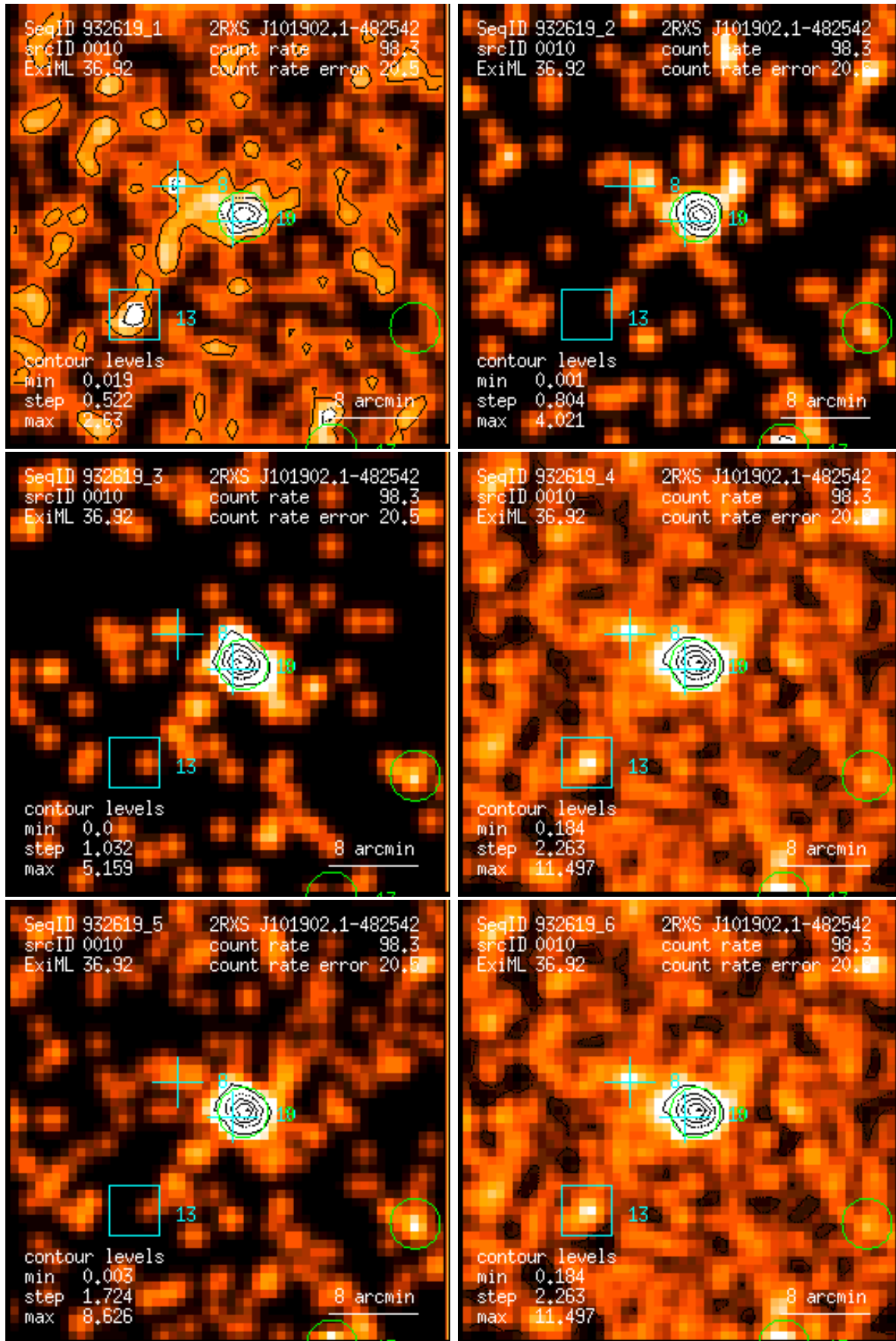
Figure 10: RASS 932619: detection 0010: band rate images, Gaussian filter: (1) PSPC channels 11 – 41, (2) 52 – 90, (3) 91 – 201, (4) 11 – 235, (5) 52 – 201, (6) 11 – 201. Broad band rates in counts/ks. Band rate contour levels in counts/ks/arcmin 2 .
