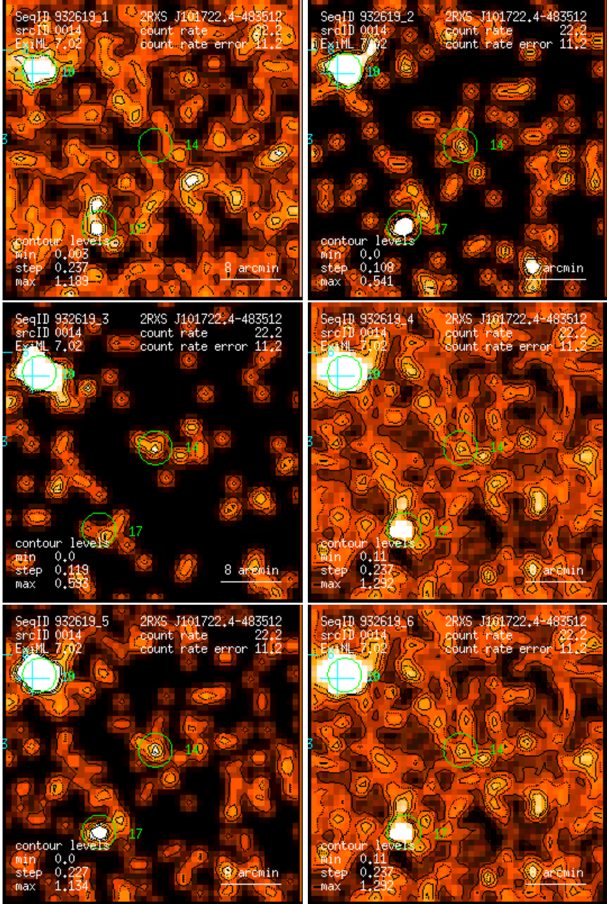
Figure 14: RASS 932619: detection 0014: band rate images, Gaussian filter: (1) PSPC channels 11 – 41, (2) 52 – 90, (3) 91 – 201, (4) 11 – 235, (5) 52 – 201, (6) 11 – 201. Broad band rates in counts/ks. Band rate contour levels in counts/ks/arcmin 2 .
