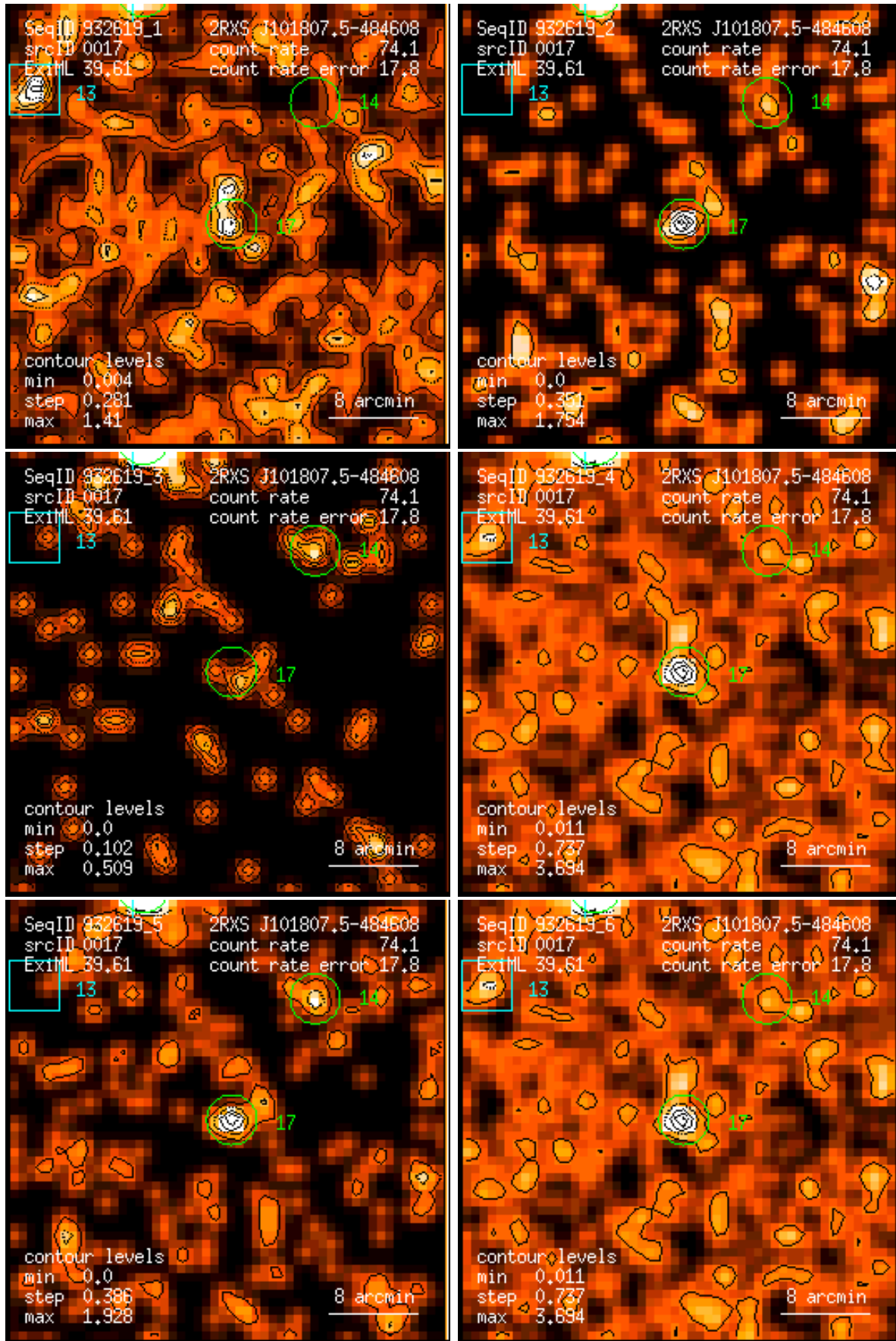
Figure 17: RASS 932619: detection 0017: band rate images, Gaussian filter: (1) PSPC channels 11 – 41, (2) 52 – 90, (3) 91 – 201, (4) 11 – 235, (5) 52 – 201, (6) 11 – 201. Broad band rates in counts/ks. Band rate contour levels in counts/ks/arcmin 2 .
