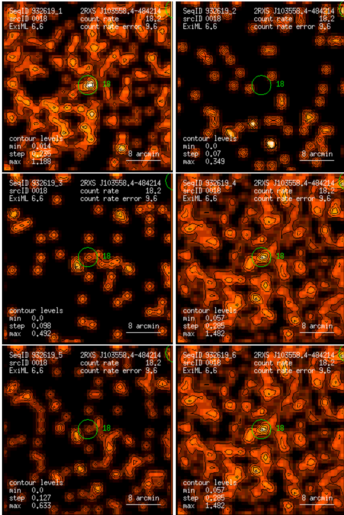
Figure 18: RASS 932619: detection 0018: band rate images, Gaussian filter: (1) PSPC channels 11 – 41, (2) 52 – 90, (3) 91 – 201, (4) 11 – 235, (5) 52 – 201, (6) 11 – 201. Broad band rates in counts/ks. Band rate contour levels in counts/ks/arcmin 2 .
