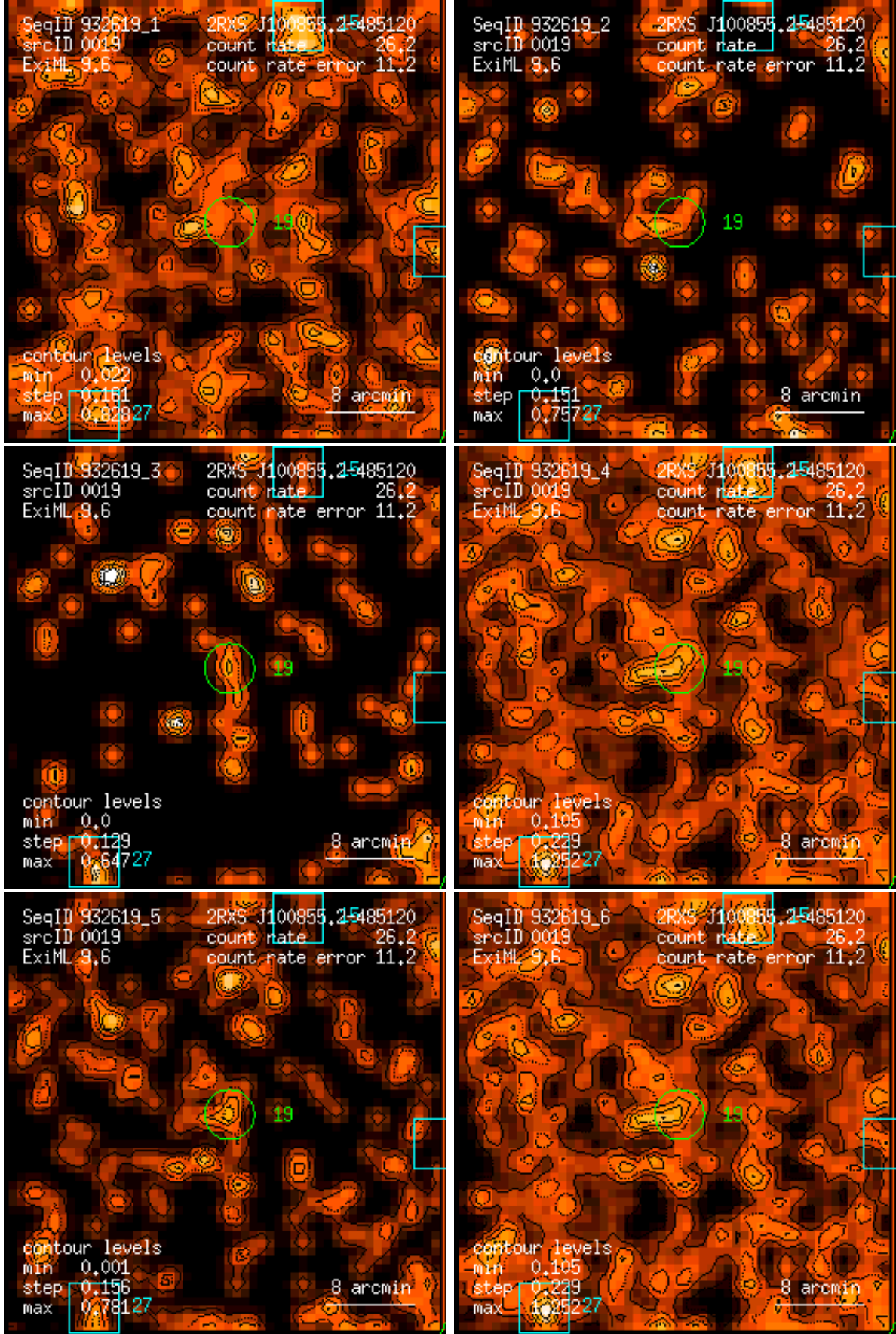
Figure 19: RASS 932619: detection 0019: band rate images, Gaussian filter: (1) PSPC channels 11 – 41, (2) 52 – 90, (3) 91 – 201, (4) 11 – 235, (5) 52 – 201, (6) 11 – 201. Broad band rates in counts/ks. Band rate contour levels in counts/ks/arcmin 2 .
