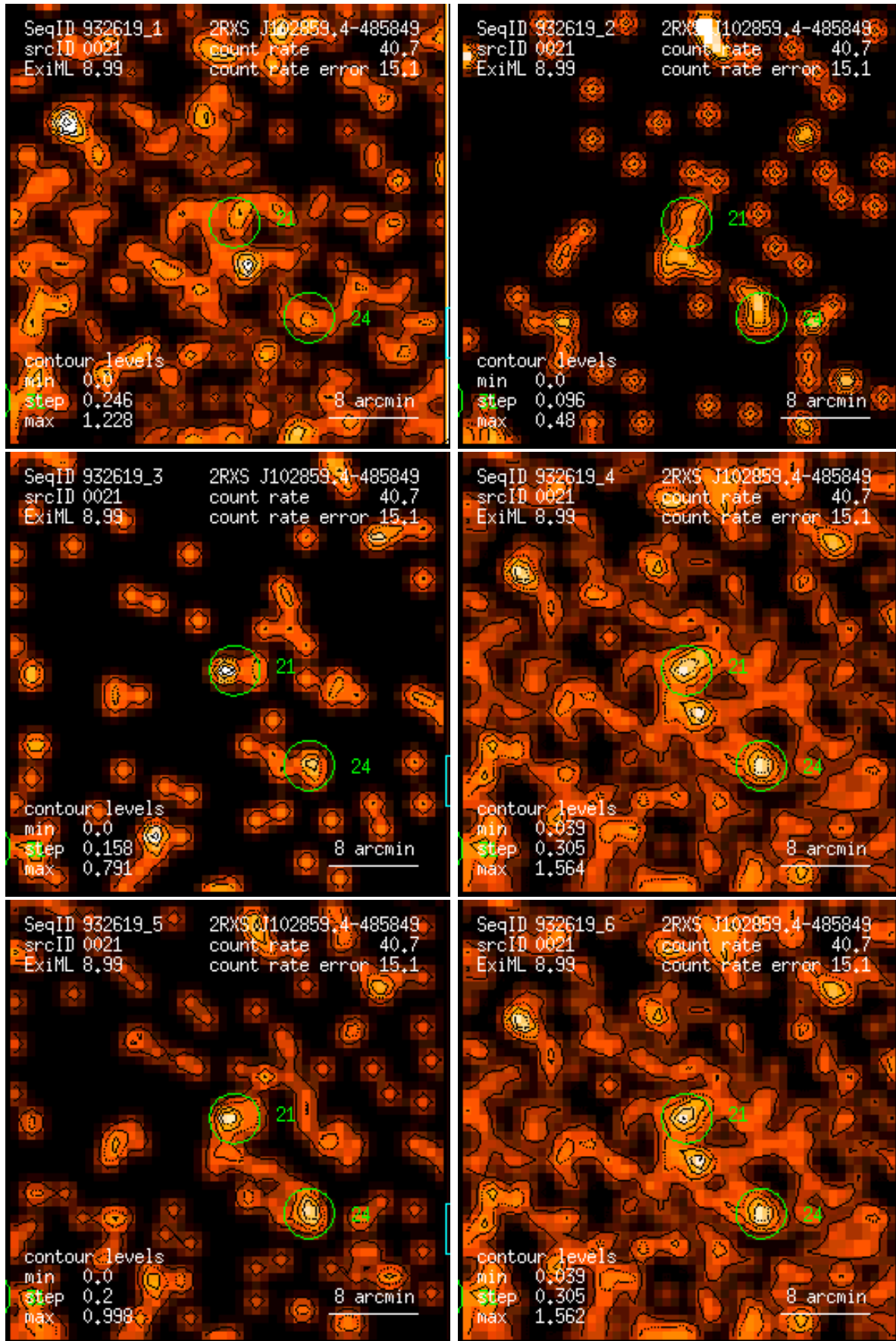
Figure 21: RASS 932619: detection 0021: band rate images, Gaussian filter: (1) PSPC channels 11 – 41, (2) 52 – 90, (3) 91 – 201, (4) 11 – 235, (5) 52 – 201, (6) 11 – 201. Broad band rates in counts/ks. Band rate contour levels in counts/ks/arcmin 2 .
