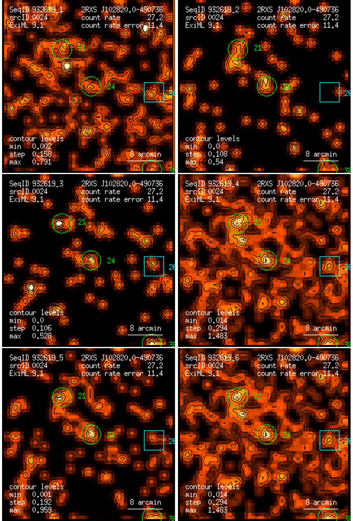
Figure 24: RASS 932619: detection 0024: band rate images, Gaussian filter: (1) PSPC channels 11 – 41, (2) 52 – 90, (3) 91 – 201, (4) 11 – 235, (5) 52 – 201, (6) 11 – 201. Broad band rates in counts/ks. Band rate contour levels in counts/ks/arcmin 2 .
