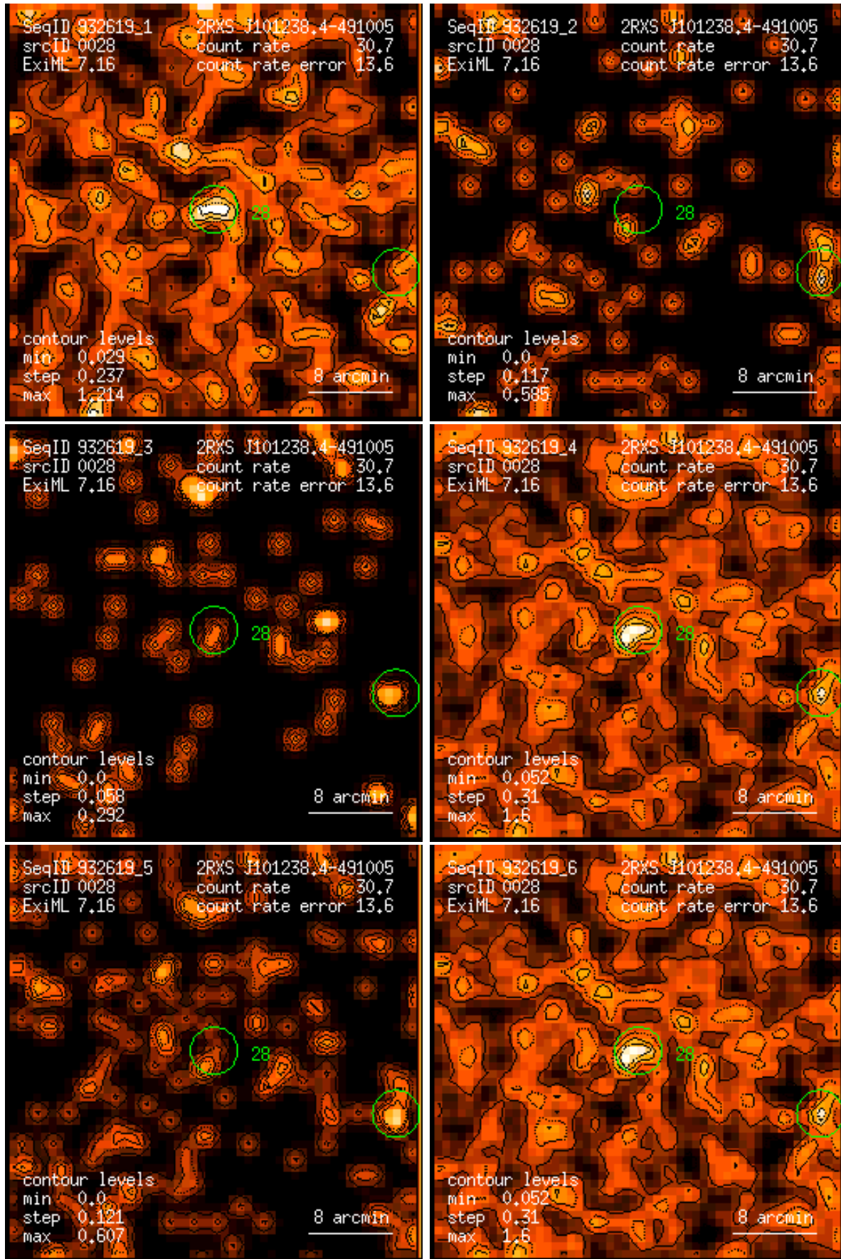
Figure 28: RASS 932619: detection 0028: band rate images, Gaussian filter: (1) PSPC channels 11 – 41, (2) 52 – 90, (3) 91 – 201, (4) 11 – 235, (5) 52 – 201, (6) 11 – 201. Broad band rates in counts/ks. Band rate contour levels in counts/ks/arcmin 2 .
