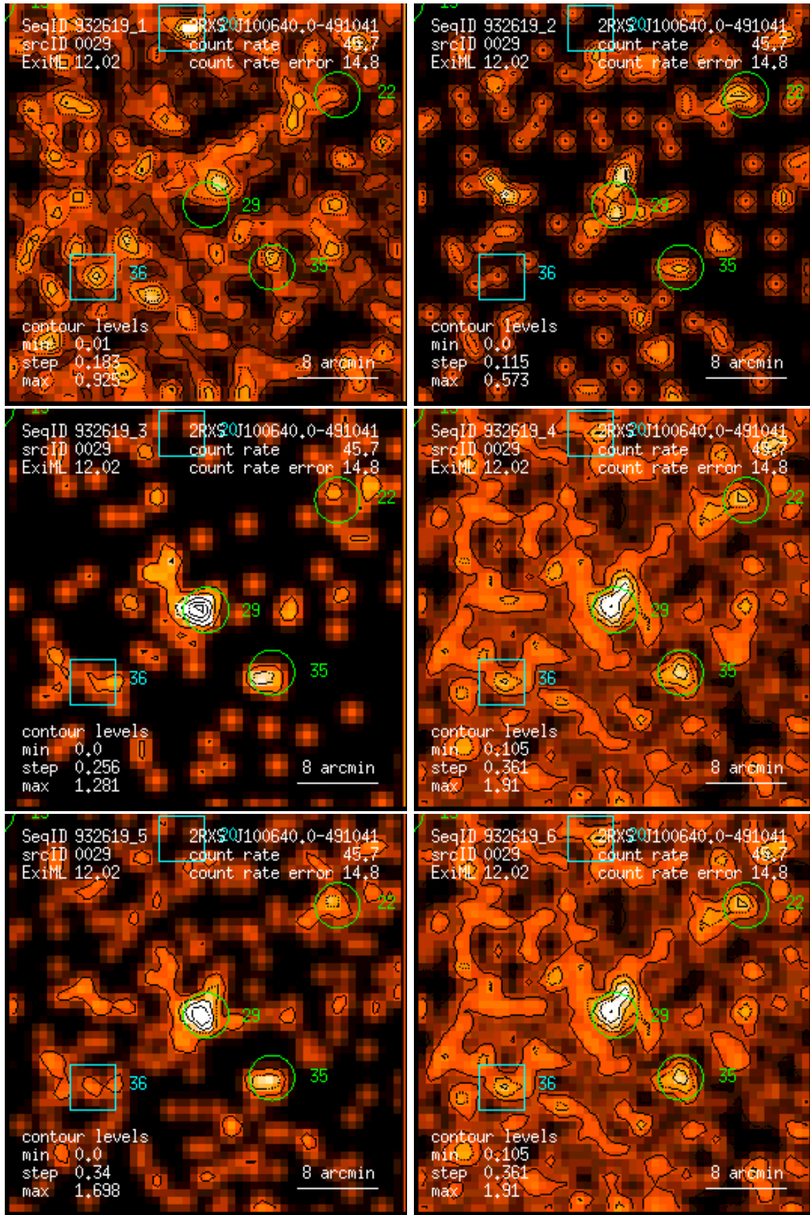
Figure 29: RASS 932619: detection 0029: band rate images, Gaussian filter: (1) PSPC channels 11 – 41, (2) 52 – 90, (3) 91 – 201, (4) 11 – 235, (5) 52 – 201, (6) 11 – 201. Broad band rates in counts/ks. Band rate contour levels in counts/ks/arcmin 2 .
