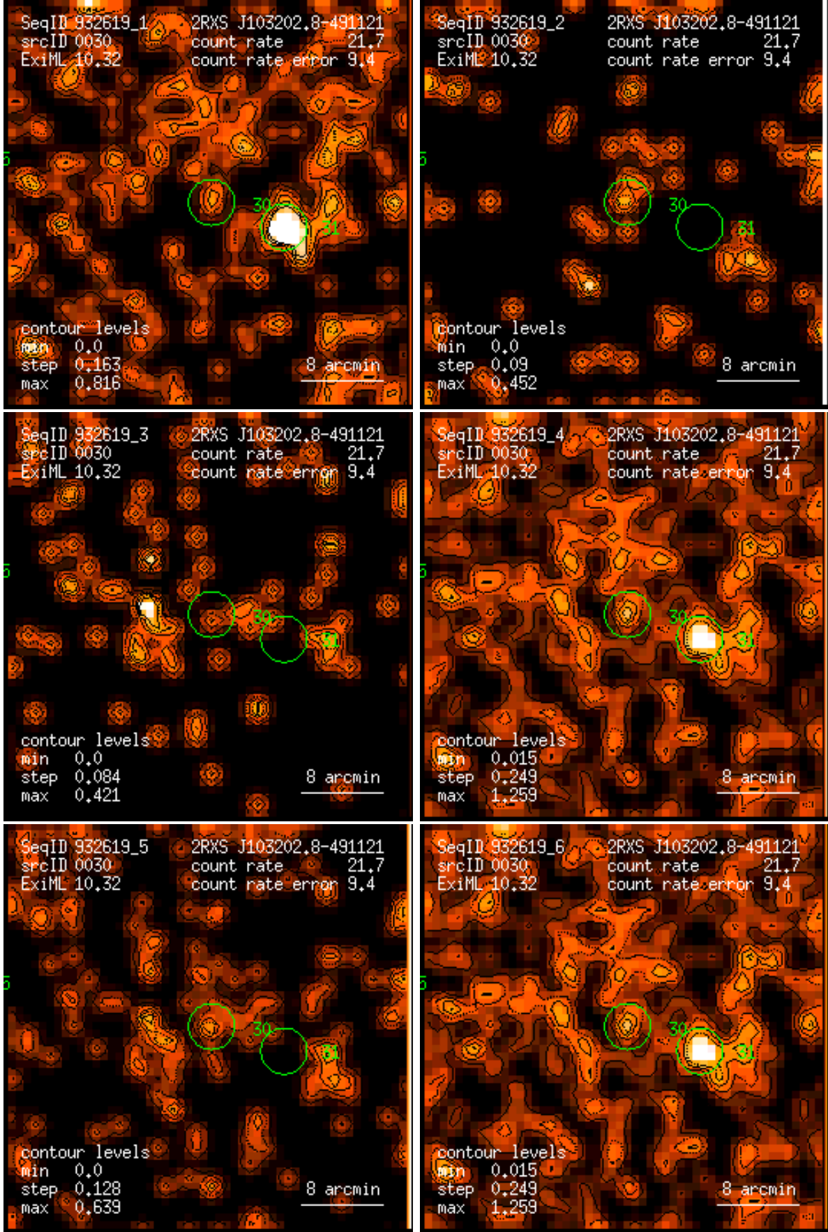
Figure 30: RASS 932619: detection 0030: band rate images, Gaussian filter: (1) PSPC channels 11 – 41, (2) 52 – 90, (3) 91 – 201, (4) 11 – 235, (5) 52 – 201, (6) 11 – 201. Broad band rates in counts/ks. Band rate contour levels in counts/ks/arcmin 2 .
