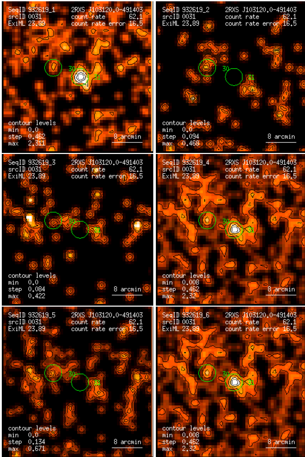
Figure 31: RASS 932619: detection 0031: band rate images, Gaussian filter: (1) PSPC channels 11 – 41, (2) 52 – 90, (3) 91 – 201, (4) 11 – 235, (5) 52 – 201, (6) 11 – 201. Broad band rates in counts/ks. Band rate contour levels in counts/ks/arcmin 2 .
