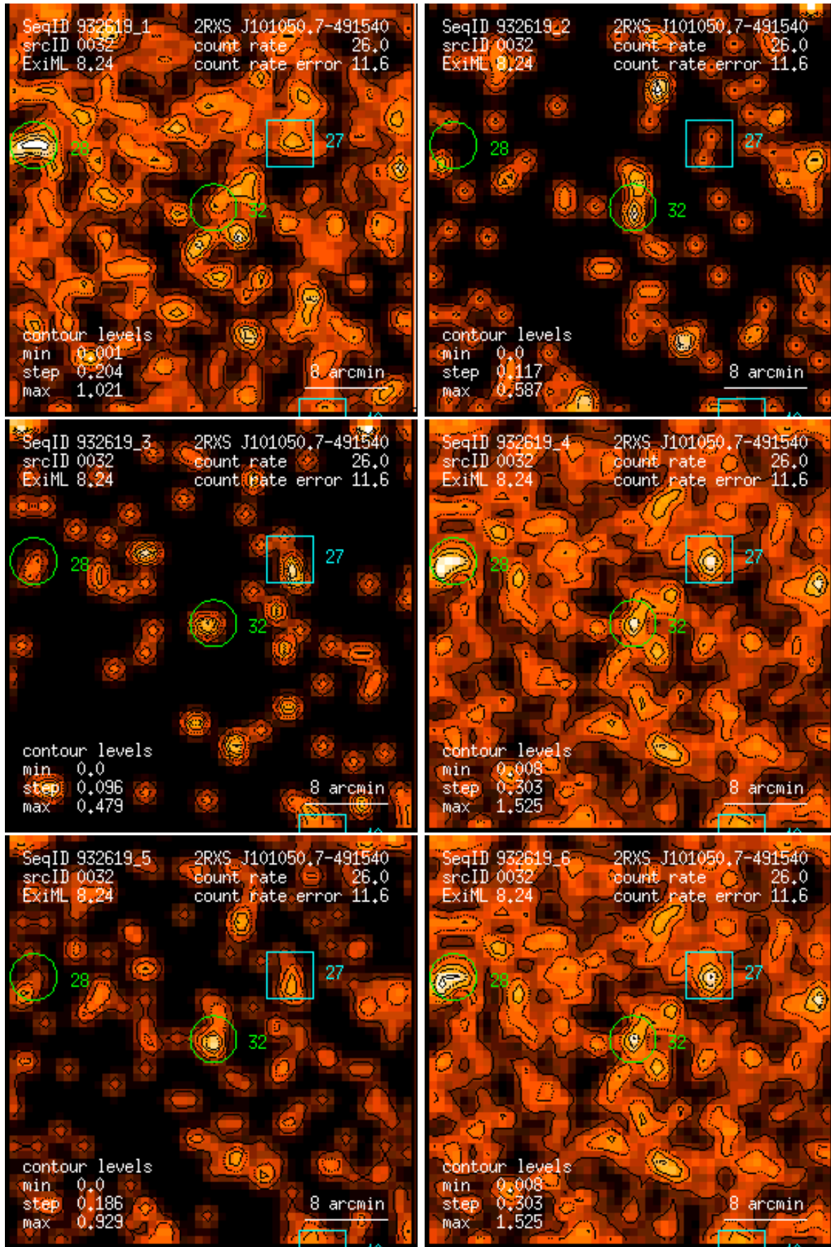
Figure 32: RASS 932619: detection 0032: band rate images, Gaussian filter: (1) PSPC channels 11 – 41, (2) 52 – 90, (3) 91 – 201, (4) 11 – 235, (5) 52 – 201, (6) 11 – 201. Broad band rates in counts/ks. Band rate contour levels in counts/ks/arcmin 2 .
