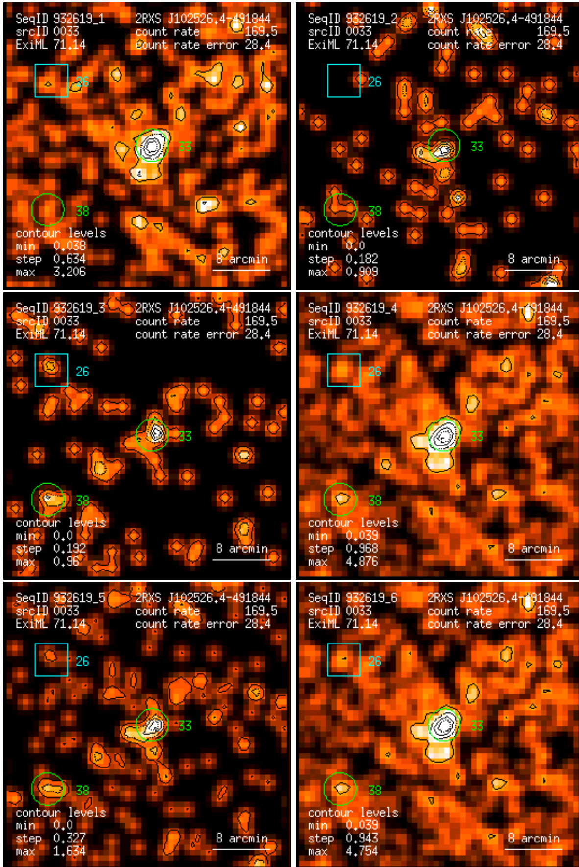
Figure 33: RASS 932619: detection 0033: band rate images, Gaussian filter: (1) PSPC channels 11 – 41, (2) 52 – 90, (3) 91 – 201, (4) 11 – 235, (5) 52 – 201, (6) 11 – 201. Broad band rates in counts/ks. Band rate contour levels in counts/ks/arcmin 2 .
