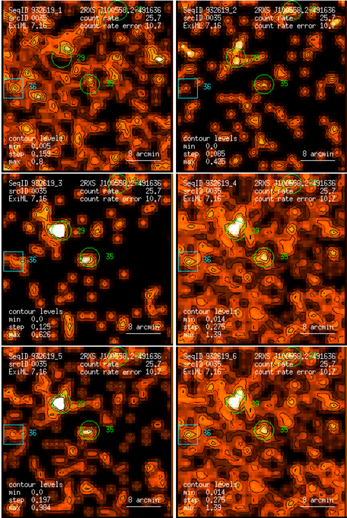
Figure 35: RASS 932619: detection 0035: band rate images, Gaussian filter: (1) PSPC channels 11 – 41, (2) 52 – 90, (3) 91 – 201, (4) 11 – 235, (5) 52 – 201, (6) 11 – 201. Broad band rates in counts/ks. Band rate contour levels in counts/ks/arcmin 2 .
