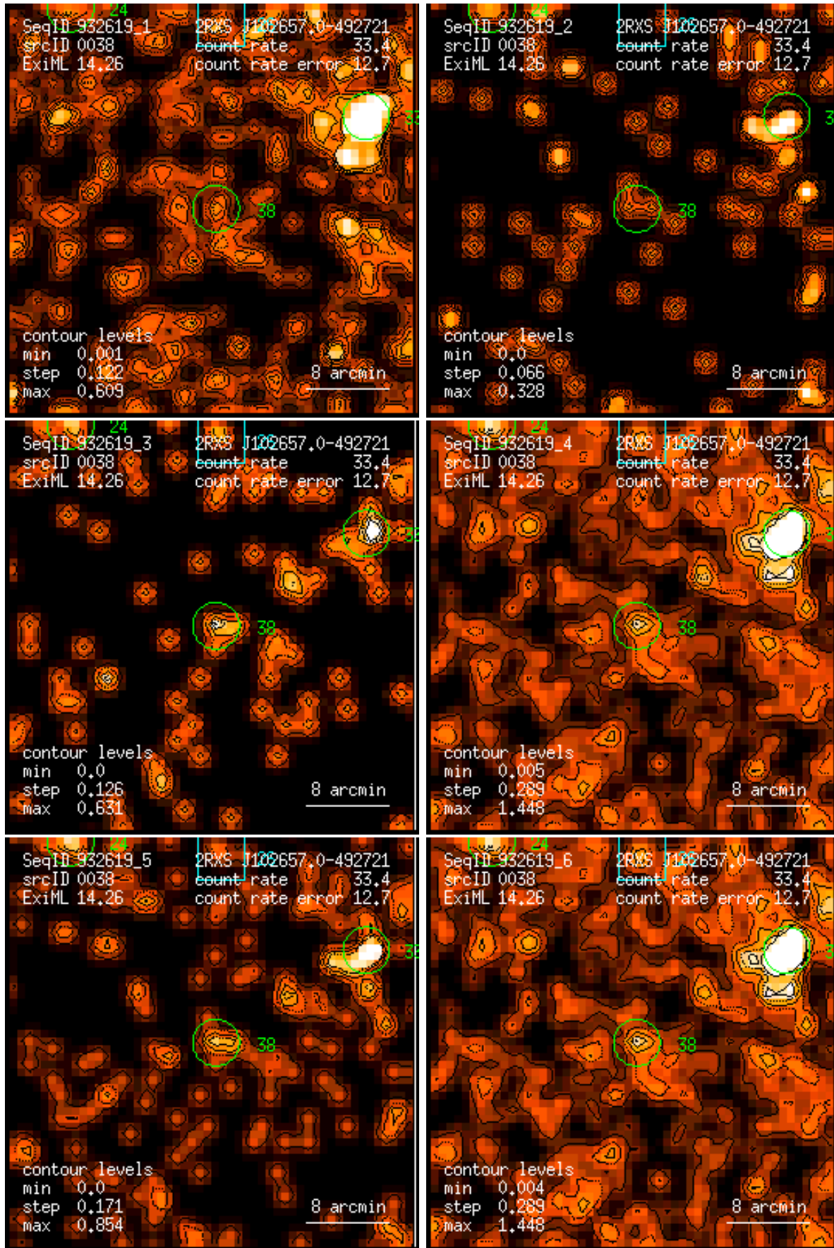
Figure 38: RASS 932619: detection 0038: band rate images, Gaussian filter: (1) PSPC channels 11 – 41, (2) 52 – 90, (3) 91 – 201, (4) 11 – 235, (5) 52 – 201, (6) 11 – 201. Broad band rates in counts/ks. Band rate contour levels in counts/ks/arcmin 2 .
