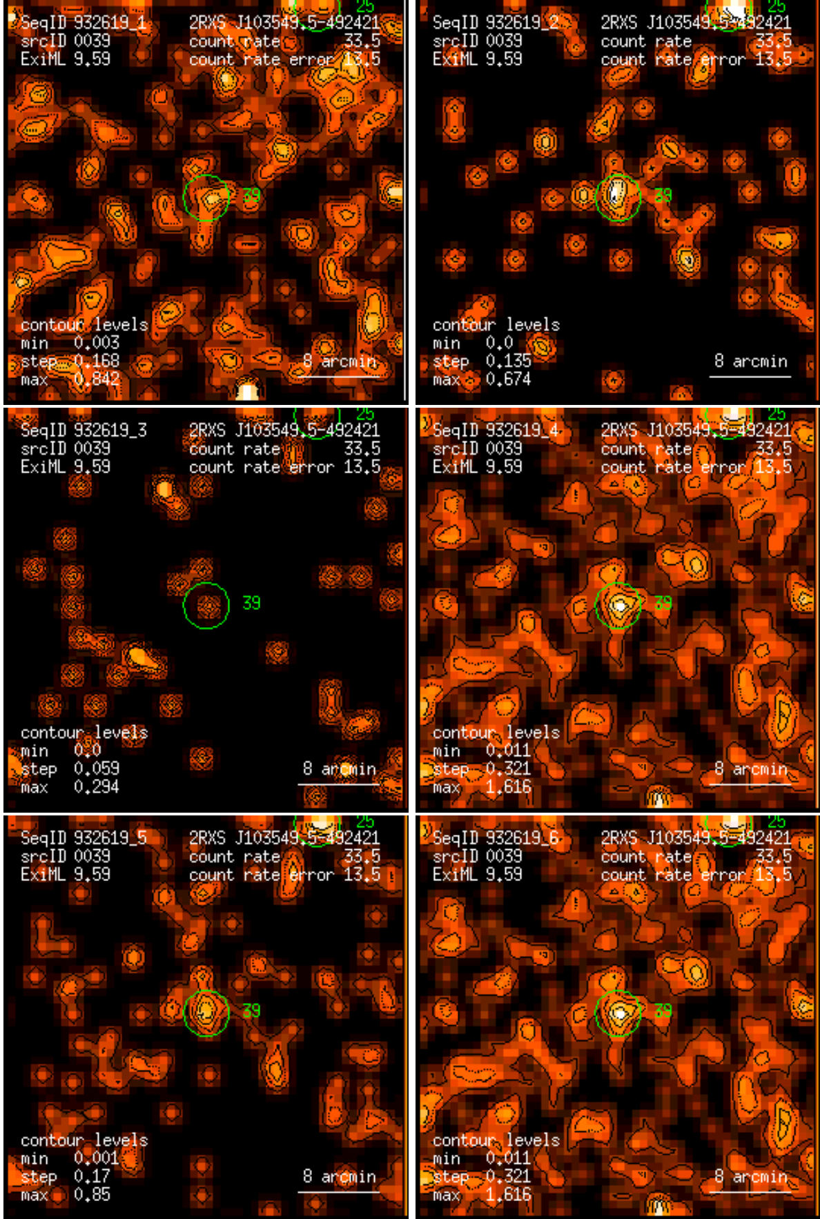
Figure 39: RASS 932619: detection 0039: band rate images, Gaussian filter: (1) PSPC channels 11 – 41, (2) 52 – 90, (3) 91 – 201, (4) 11 – 235, (5) 52 – 201, (6) 11 – 201. Broad band rates in counts/ks. Band rate contour levels in counts/ks/arcmin 2 .
