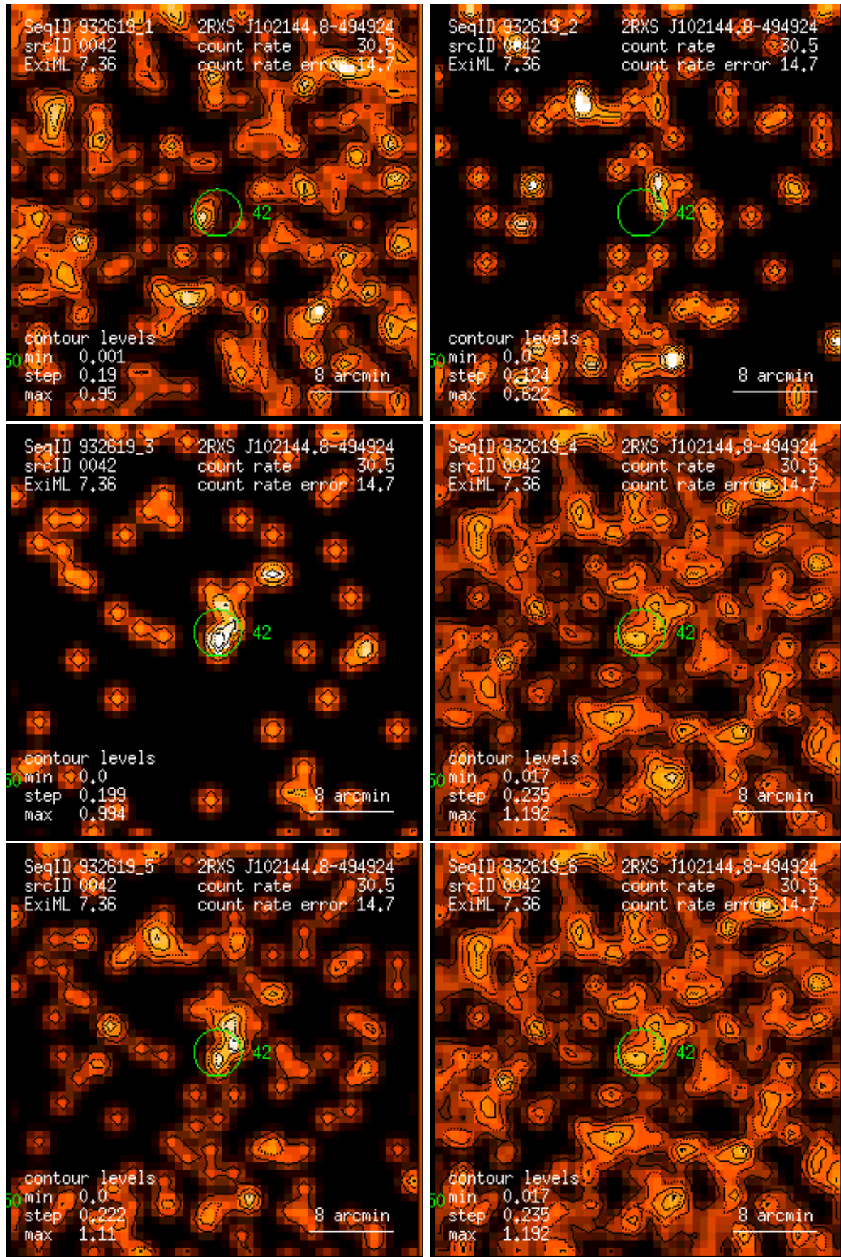
Figure 42: RASS 932619: detection 0042: band rate images, Gaussian filter: (1) PSPC channels 11 – 41, (2) 52 – 90, (3) 91 – 201, (4) 11 – 235, (5) 52 – 201, (6) 11 – 201. Broad band rates in counts/ks. Band rate contour levels in counts/ks/arcmin 2 .
