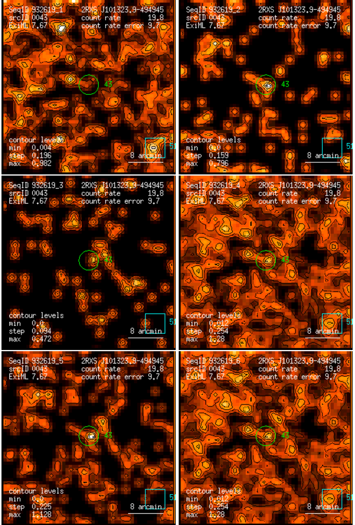
Figure 43: RASS 932619: detection 0043: band rate images, Gaussian filter: (1) PSPC channels 11 – 41, (2) 52 – 90, (3) 91 – 201, (4) 11 – 235, (5) 52 – 201, (6) 11 – 201. Broad band rates in counts/ks. Band rate contour levels in counts/ks/arcmin 2 .
