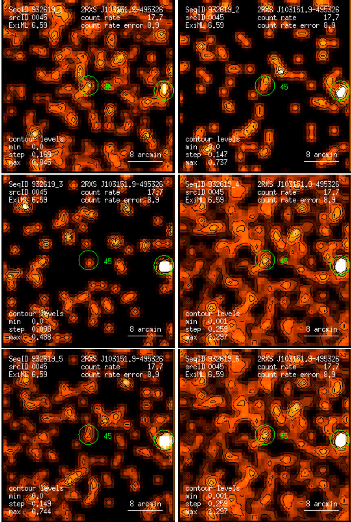
Figure 45: RASS 932619: detection 0045: band rate images, Gaussian filter: (1) PSPC channels 11 – 41, (2) 52 – 90, (3) 91 – 201, (4) 11 – 235, (5) 52 – 201, (6) 11 – 201. Broad band rates in counts/ks. Band rate contour levels in counts/ks/arcmin 2 .
