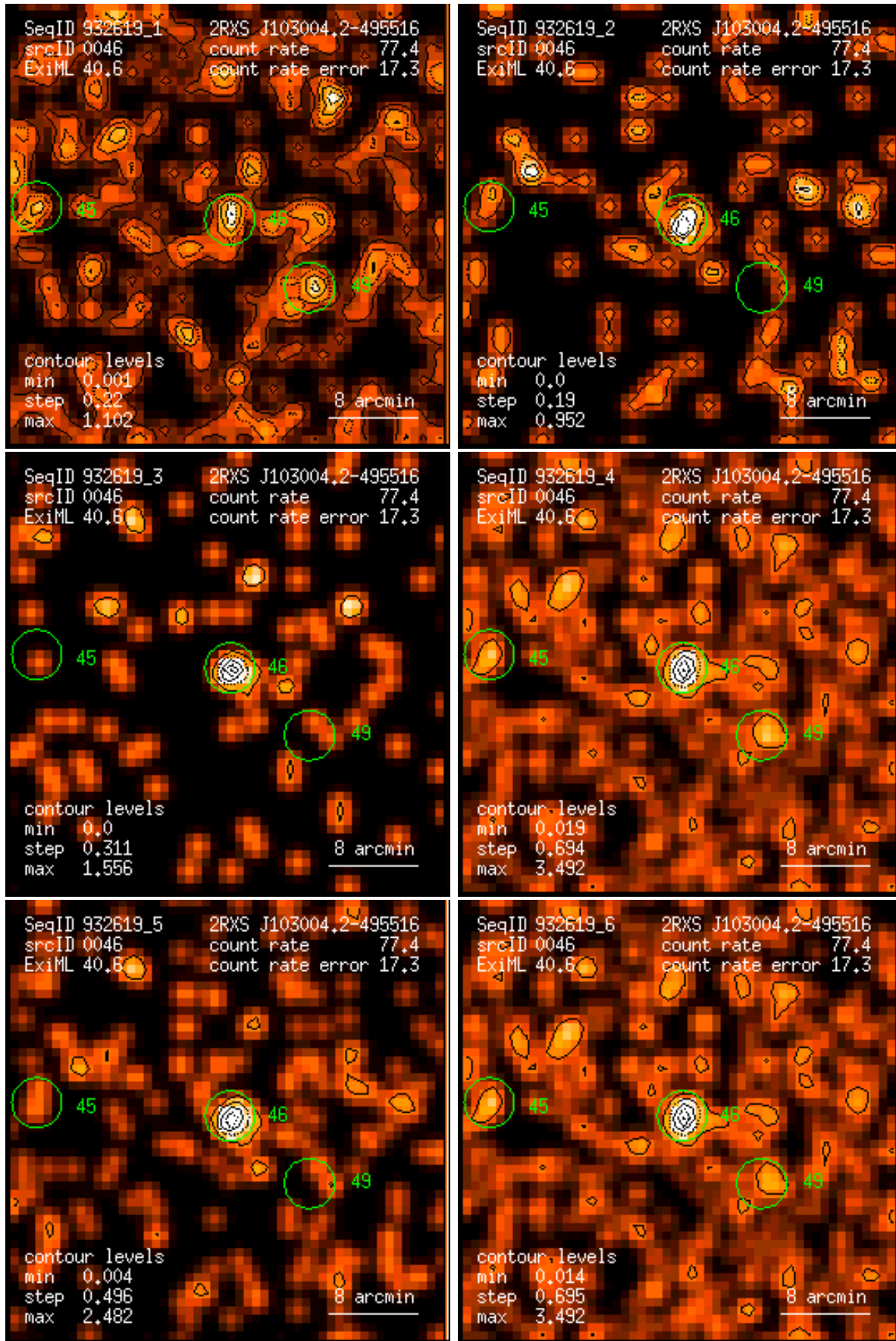
Figure 46: RASS 932619: detection 0046: band rate images, Gaussian filter: (1) PSPC channels 11 – 41, (2) 52 – 90, (3) 91 – 201, (4) 11 – 235, (5) 52 – 201, (6) 11 – 201. Broad band rates in counts/ks. Band rate contour levels in counts/ks/arcmin 2 .
