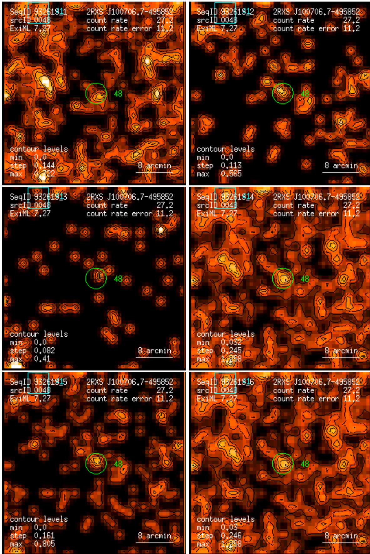
Figure 48: RASS 932619: detection 0048: band rate images, Gaussian filter: (1) PSPC channels 11 – 41, (2) 52 – 90, (3) 91 – 201, (4) 11 – 235, (5) 52 – 201, (6) 11 – 201. Broad band rates in counts/ks. Band rate contour levels in counts/ks/arcmin 2 .
