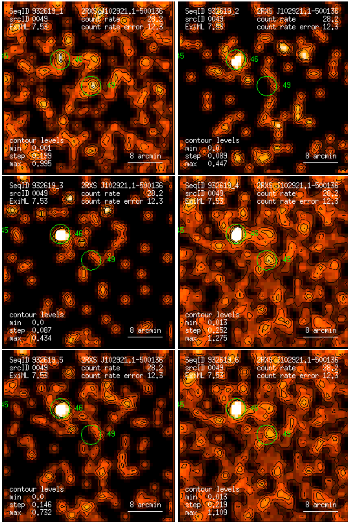
Figure 49: RASS 932619: detection 0049: band rate images, Gaussian filter: (1) PSPC channels 11 – 41, (2) 52 – 90, (3) 91 – 201, (4) 11 – 235, (5) 52 – 201, (6) 11 – 201. Broad band rates in counts/ks. Band rate contour levels in counts/ks/arcmin 2 .
