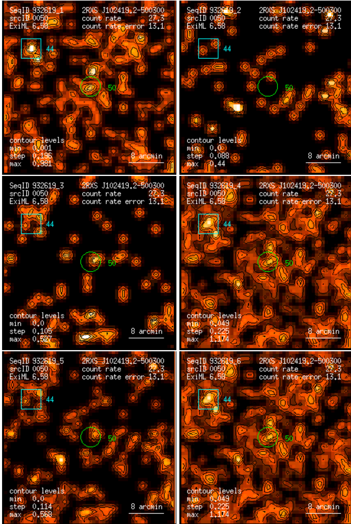
Figure 50: RASS 932619: detection 0050: band rate images, Gaussian filter: (1) PSPC channels 11 – 41, (2) 52 – 90, (3) 91 – 201, (4) 11 – 235, (5) 52 – 201, (6) 11 – 201. Broad band rates in counts/ks. Band rate contour levels in counts/ks/arcmin 2 .
