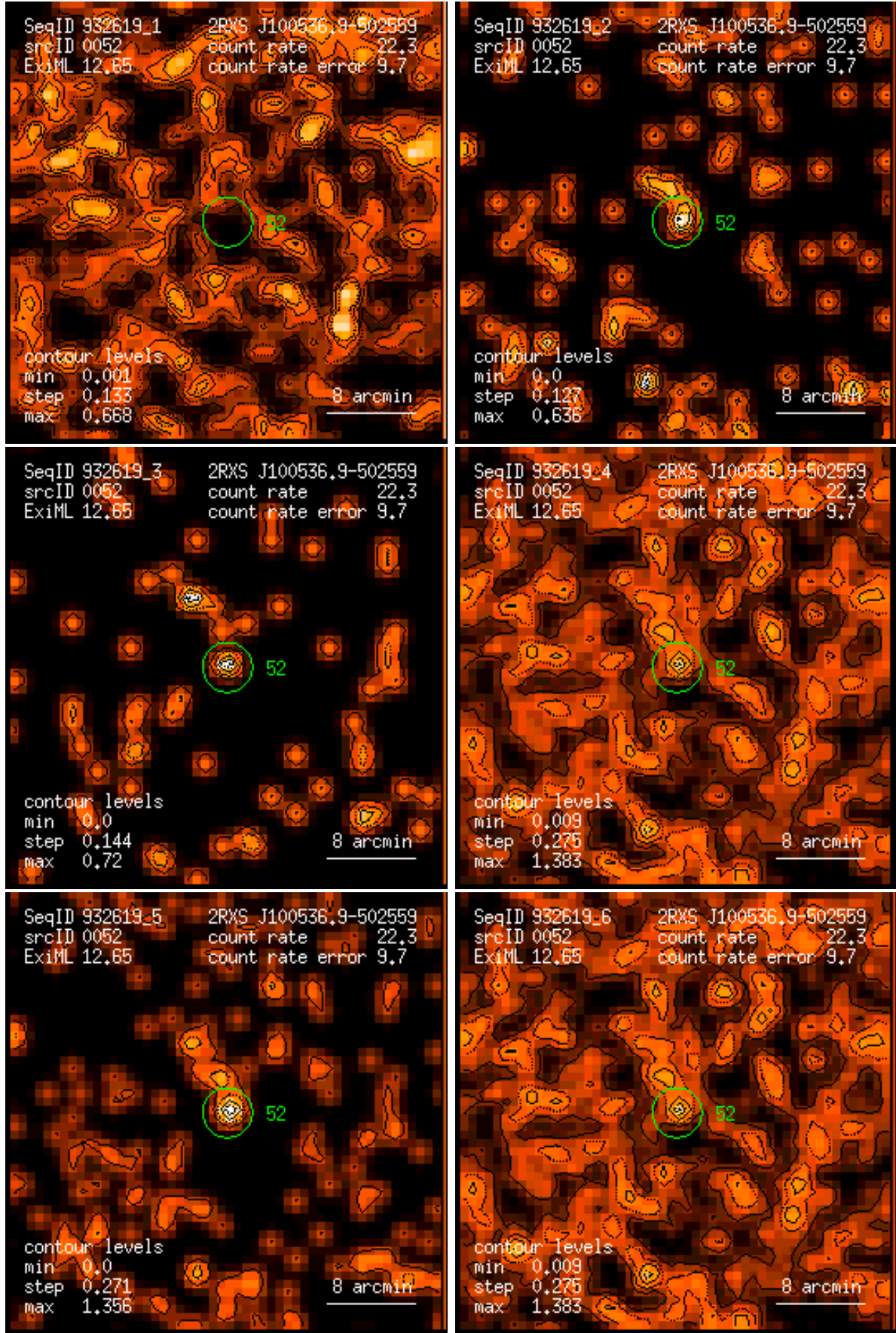
Figure 52: RASS 932619: detection 0052: band rate images, Gaussian filter: (1) PSPC channels 11 – 41, (2) 52 – 90, (3) 91 – 201, (4) 11 – 235, (5) 52 – 201, (6) 11 – 201. Broad band rates in counts/ks. Band rate contour levels in counts/ks/arcmin 2 .
