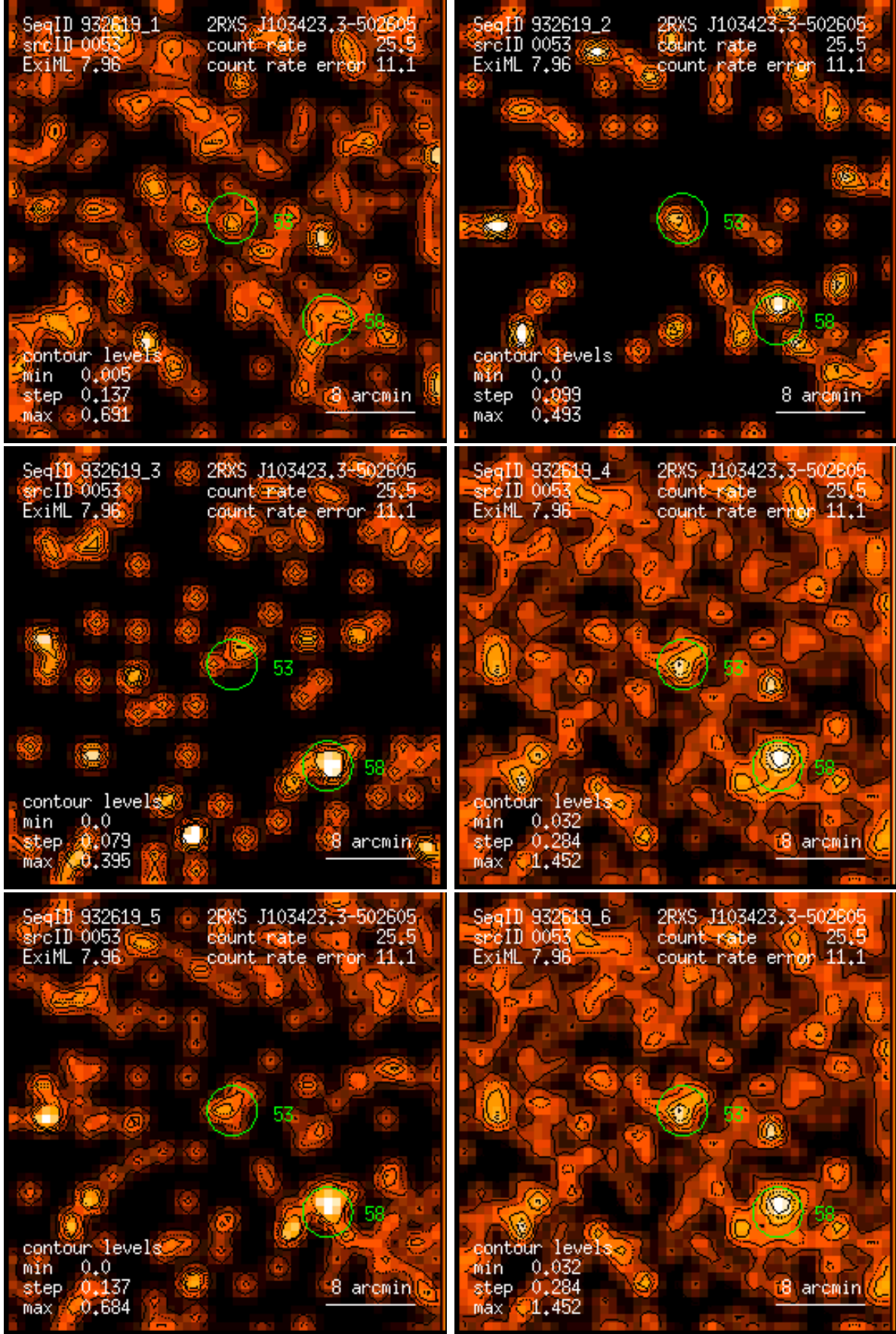
Figure 53: RASS 932619: detection 0053: band rate images, Gaussian filter: (1) PSPC channels 11 – 41, (2) 52 – 90, (3) 91 – 201, (4) 11 – 235, (5) 52 – 201, (6) 11 – 201. Broad band rates in counts/ks. Band rate contour levels in counts/ks/arcmin 2 .
