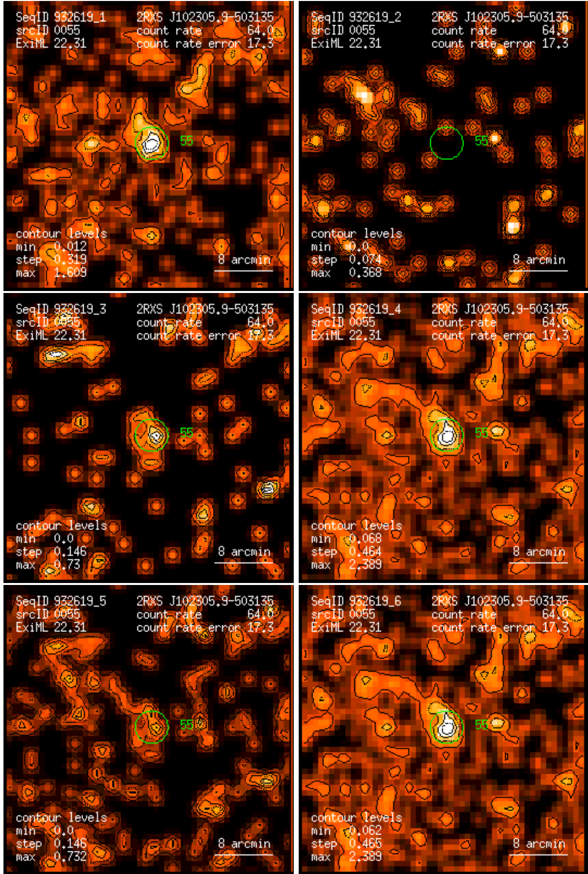
Figure 55: RASS 932619: detection 0055: band rate images, Gaussian filter: (1) PSPC channels 11 – 41, (2) 52 – 90, (3) 91 – 201, (4) 11 – 235, (5) 52 – 201, (6) 11 – 201. Broad band rates in counts/ks. Band rate contour levels in counts/ks/arcmin 2 .
