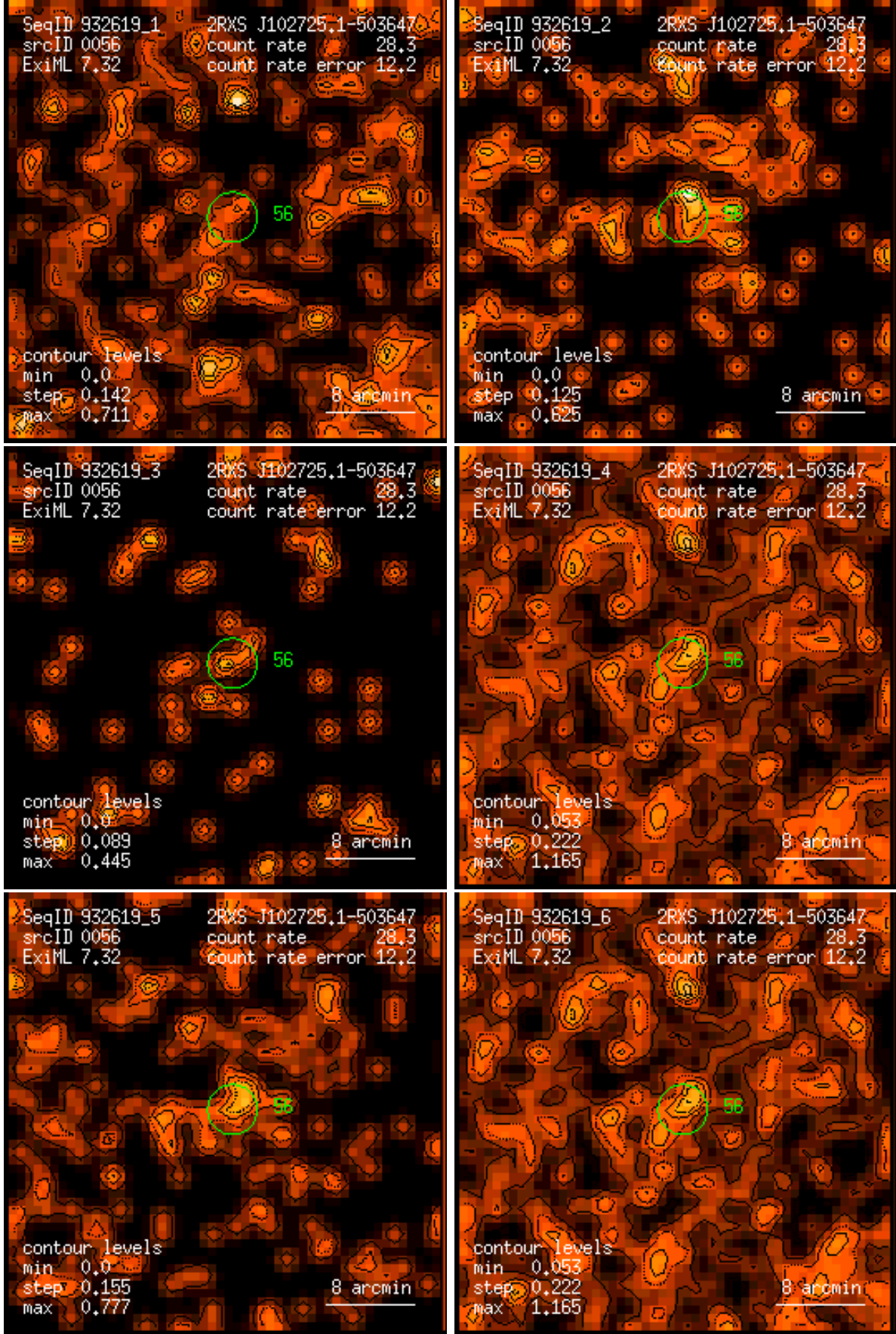
Figure 56: RASS 932619: detection 0056: band rate images, Gaussian filter: (1) PSPC channels 11 – 41, (2) 52 – 90, (3) 91 – 201, (4) 11 – 235, (5) 52 – 201, (6) 11 – 201. Broad band rates in counts/ks. Band rate contour levels in counts/ks/arcmin 2 .
