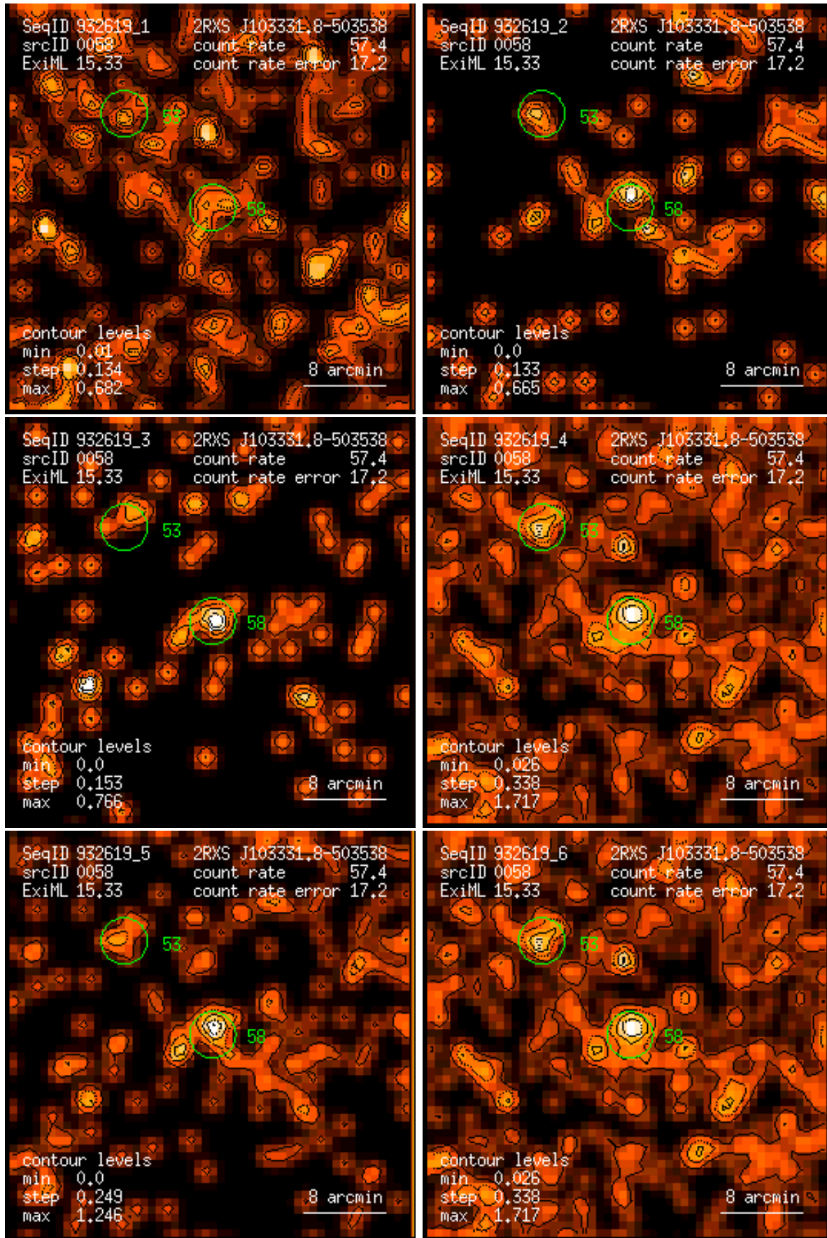
Figure 58: RASS 932619: detection 0058: band rate images, Gaussian filter: (1) PSPC channels 11 – 41, (2) 52 – 90, (3) 91 – 201, (4) 11 – 235, (5) 52 – 201, (6) 11 – 201. Broad band rates in counts/ks. Band rate contour levels in counts/ks/arcmin 2 .
