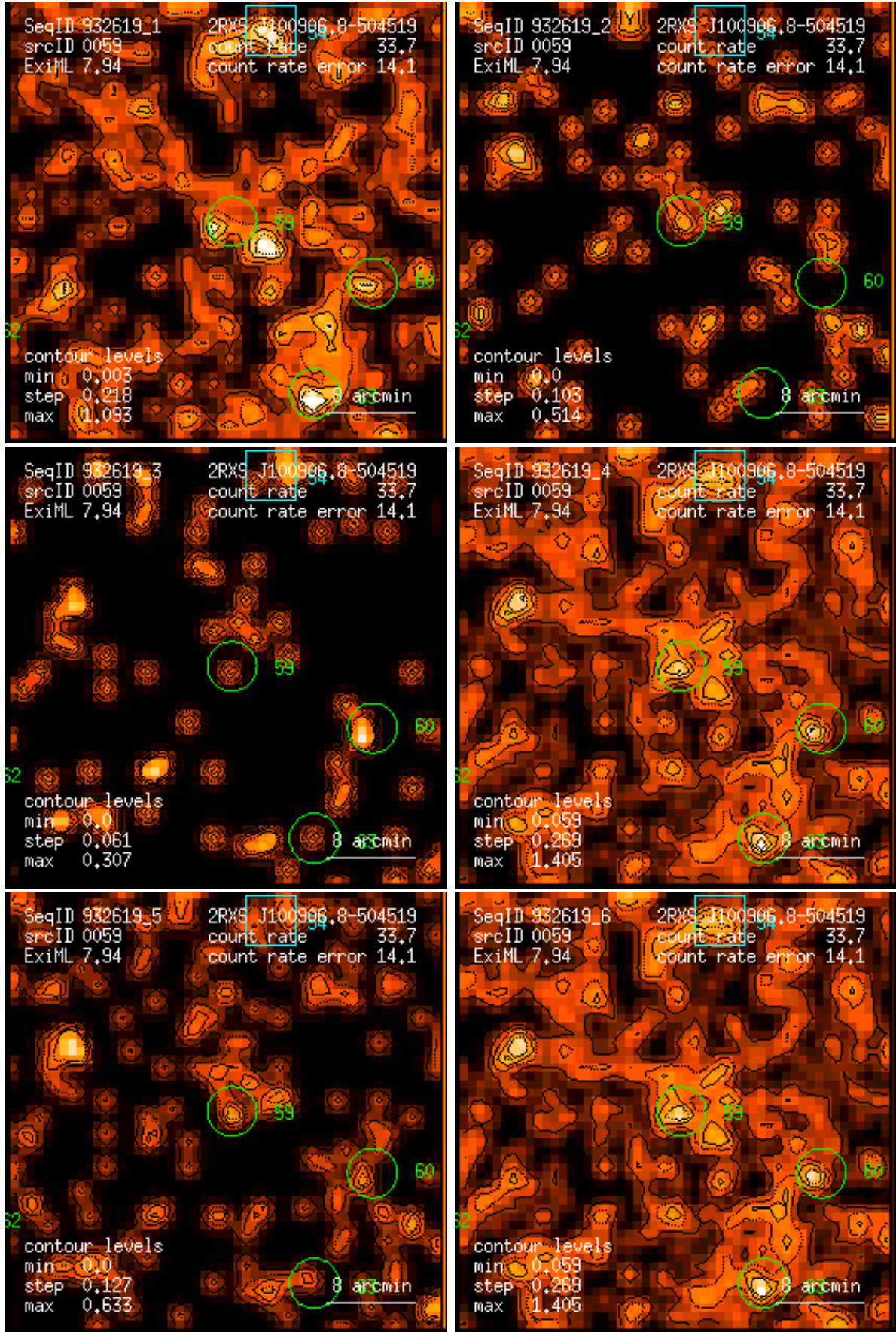
Figure 59: RASS 932619: detection 0059: band rate images, Gaussian filter: (1) PSPC channels 11 – 41, (2) 52 – 90, (3) 91 – 201, (4) 11 – 235, (5) 52 – 201, (6) 11 – 201. Broad band rates in counts/ks. Band rate contour levels in counts/ks/arcmin 2 .
