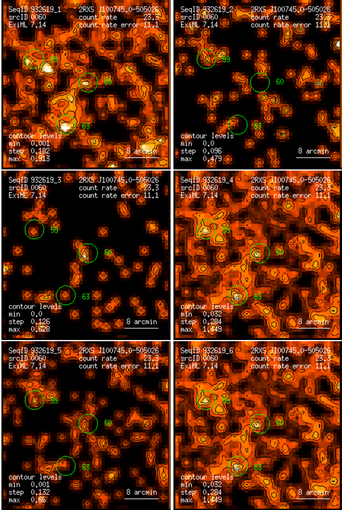
Figure 60: RASS 932619: detection 0060: band rate images, Gaussian filter: (1) PSPC channels 11 – 41, (2) 52 – 90, (3) 91 – 201, (4) 11 – 235, (5) 52 – 201, (6) 11 – 201. Broad band rates in counts/ks. Band rate contour levels in counts/ks/arcmin 2 .
