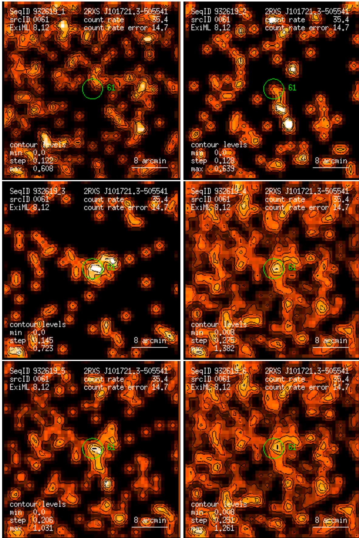
Figure 61: RASS 932619: detection 0061: band rate images, Gaussian filter: (1) PSPC channels 11 – 41, (2) 52 – 90, (3) 91 – 201, (4) 11 – 235, (5) 52 – 201, (6) 11 – 201. Broad band rates in counts/ks. Band rate contour levels in counts/ks/arcmin 2 .
