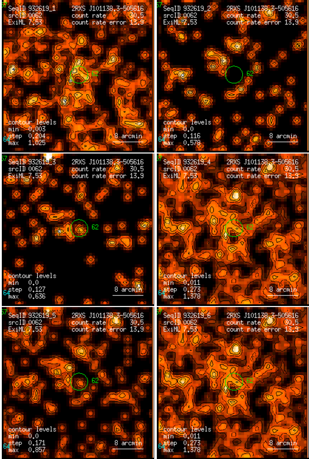
Figure 62: RASS 932619: detection 0062: band rate images, Gaussian filter: (1) PSPC channels 11 – 41, (2) 52 – 90, (3) 91 – 201, (4) 11 – 235, (5) 52 – 201, (6) 11 – 201. Broad band rates in counts/ks. Band rate contour levels in counts/ks/arcmin 2 .
