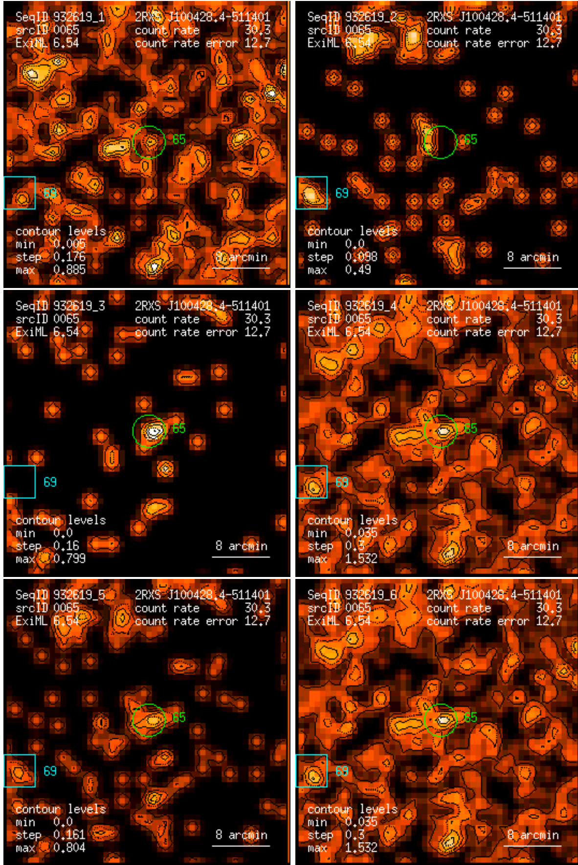
Figure 65: RASS 932619: detection 0065: band rate images, Gaussian filter: (1) PSPC channels 11 – 41, (2) 52 – 90, (3) 91 – 201, (4) 11 – 235, (5) 52 – 201, (6) 11 – 201. Broad band rates in counts/ks. Band rate contour levels in counts/ks/arcmin 2 .
